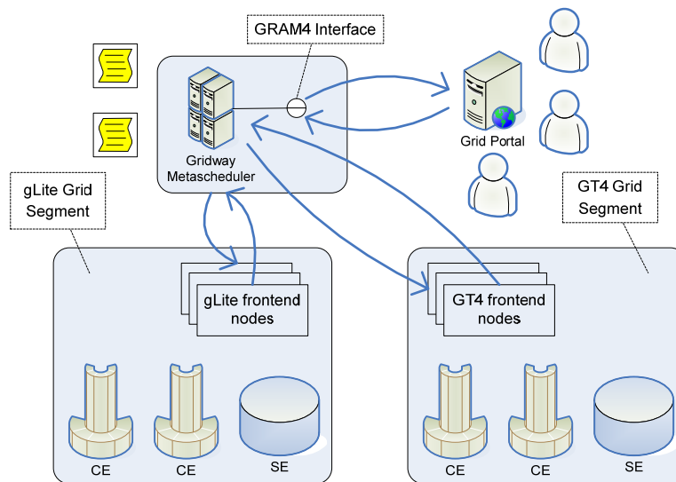
Fig. 4. Metascheduler approach
