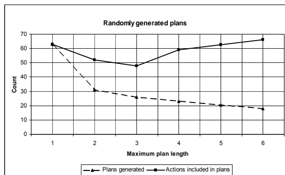
Figure 13. Number of generated plans and included actions
