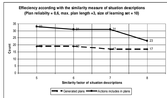
Figure 15. Number of generated plans and included actions with different T values
