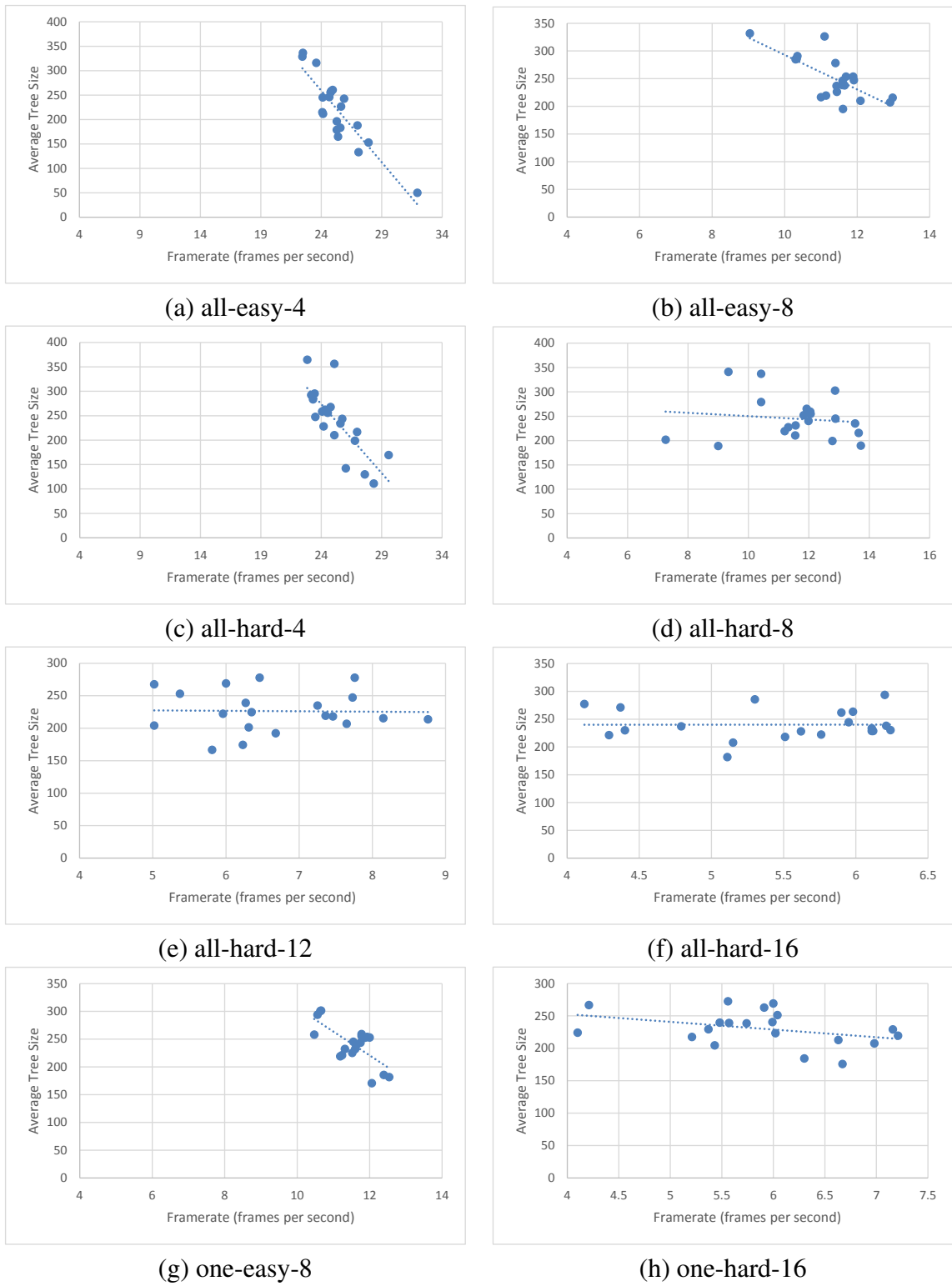
Figure 5.9: Frame rate vs. average tree size
