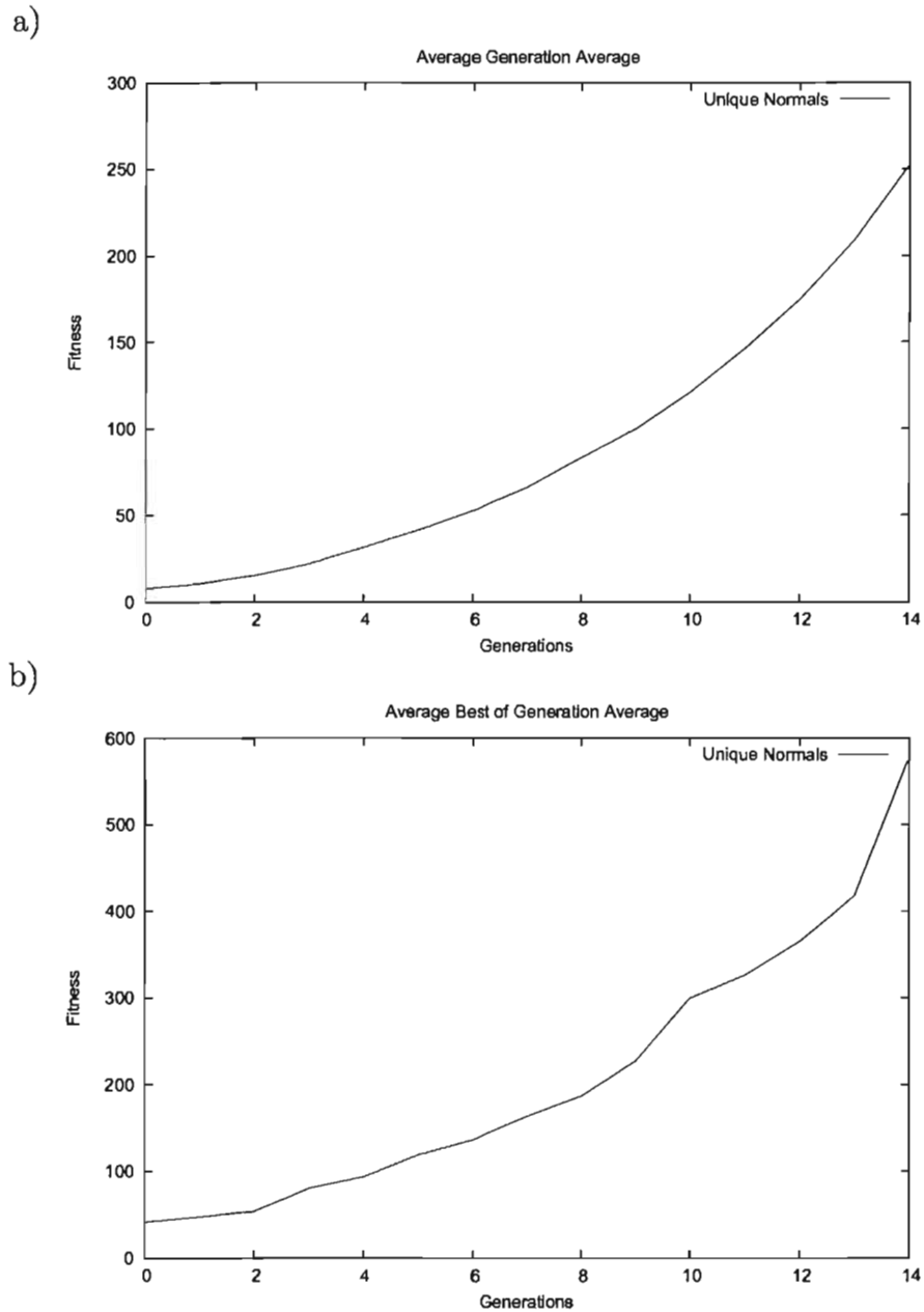
Figure 4.4: Image (a) shows the performance graph of the evolution of the maximizing unique surface normals experiment. This graph displays the average generation averaged over all 10 runs. Image (b) shows the average best of generation result during all 10 runs of the experiment.
