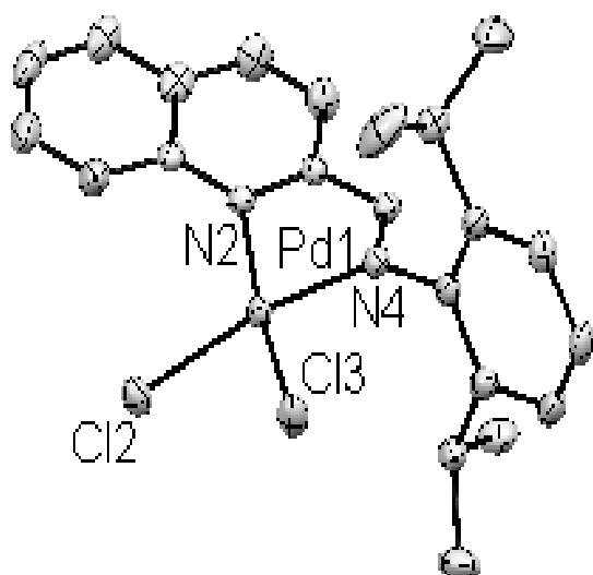
Fig. 1. X-ray crystal structure of complex 3.
