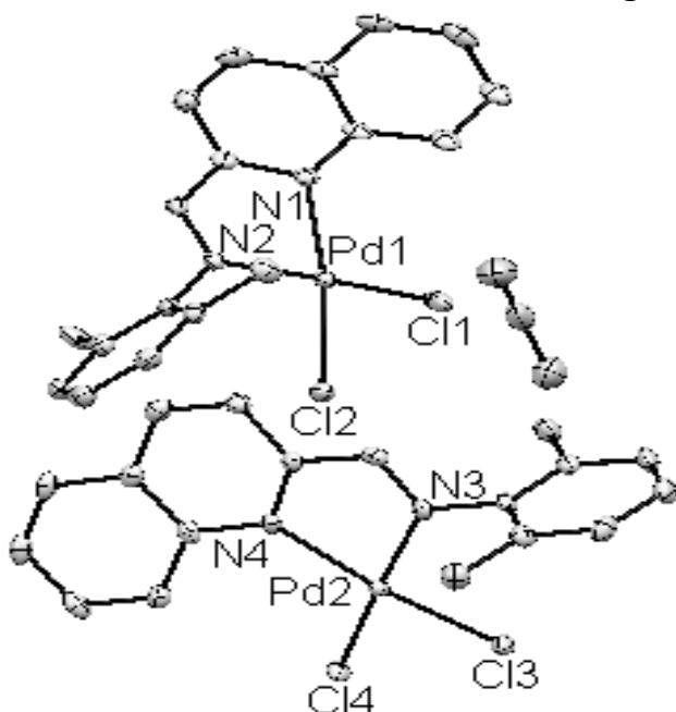
Fig. 1. X-ray crystal structure of complex 3.
