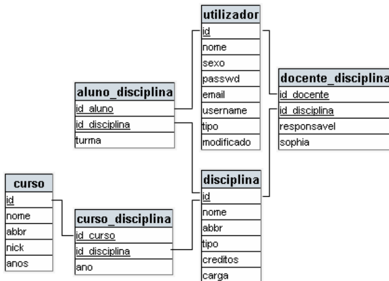
Fig. 4: Schema of the central Database
