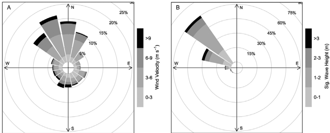
Fig. 3. – Wind and wave patterns from data collected at a meteorological station and an oceanographic buoy between 2005 and 2010 in the Sines region (SW Portugal). A) Wind velocity ( m s^{-1} ) and frequency (%) by coastal sector. B) Significant wave height (m) and frequency (%) by coastal sector.
