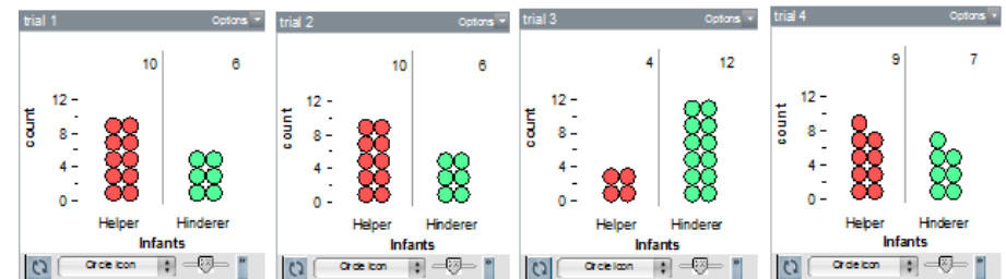
Figure 2: Outcomes of single sample simulations, under the null model, of the “Helper or Hinderer” MEA.
