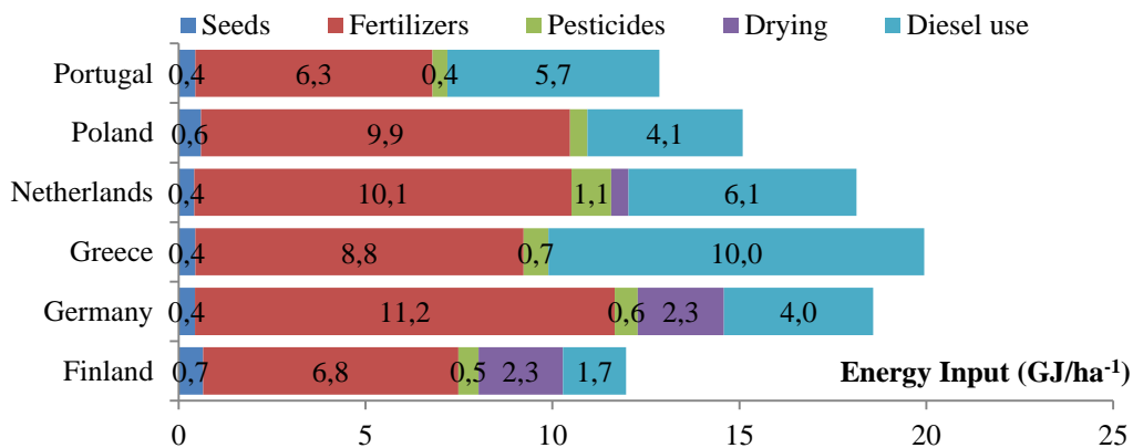
Figure 3.2. The structure of energy inputs in wheat production in GJ/ha (Gołaszewski et al., 2012)
