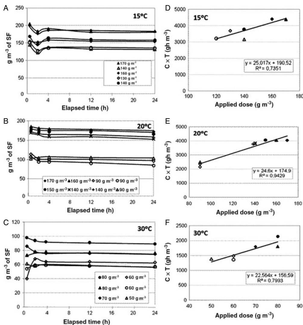
Figure 1. Parameters of the fumigation with sulfuryl fluoride (SF) of Pinus pinaster boards naturally infected with pinewood nematode Bursaphelenchus xylophilus at three temperatures. Sorption curves registered in fumigation chambers at 15 °C (A), 20 °C (B) and 30 °C (C). Relation of final CT product (concentration × time) in fumigation chambers at 15 °C (D), 20 °C (E) and 30 °C (F).
