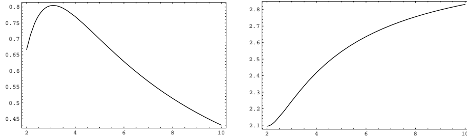
Figure 4.3: Ratio between the area occupied by the sectors and the total area of the cross-section (left) and angle opening for each sector (right).
