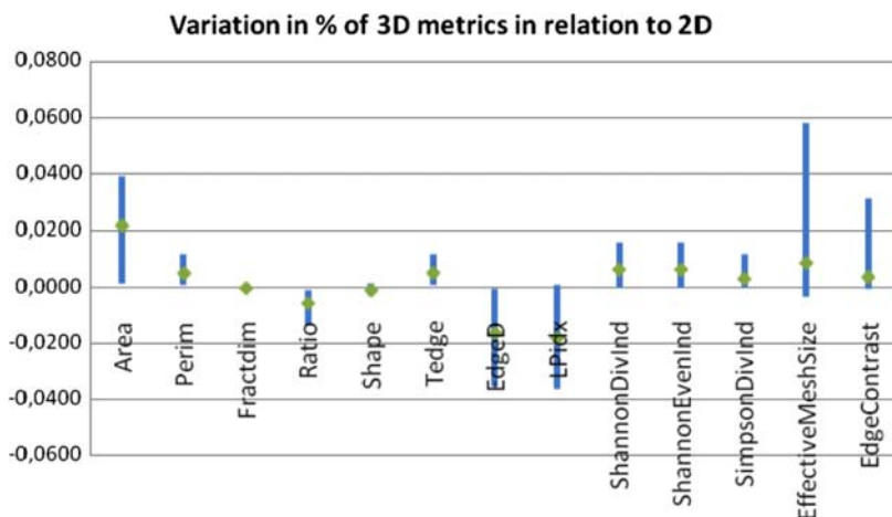
Figure 4. Variation (%) of the three-dimensional landscape metrics in relation to the planimetric calculated metrics. Figure 4. Variation (en%) des 3D métriques en relation avec les 2D métriques.
