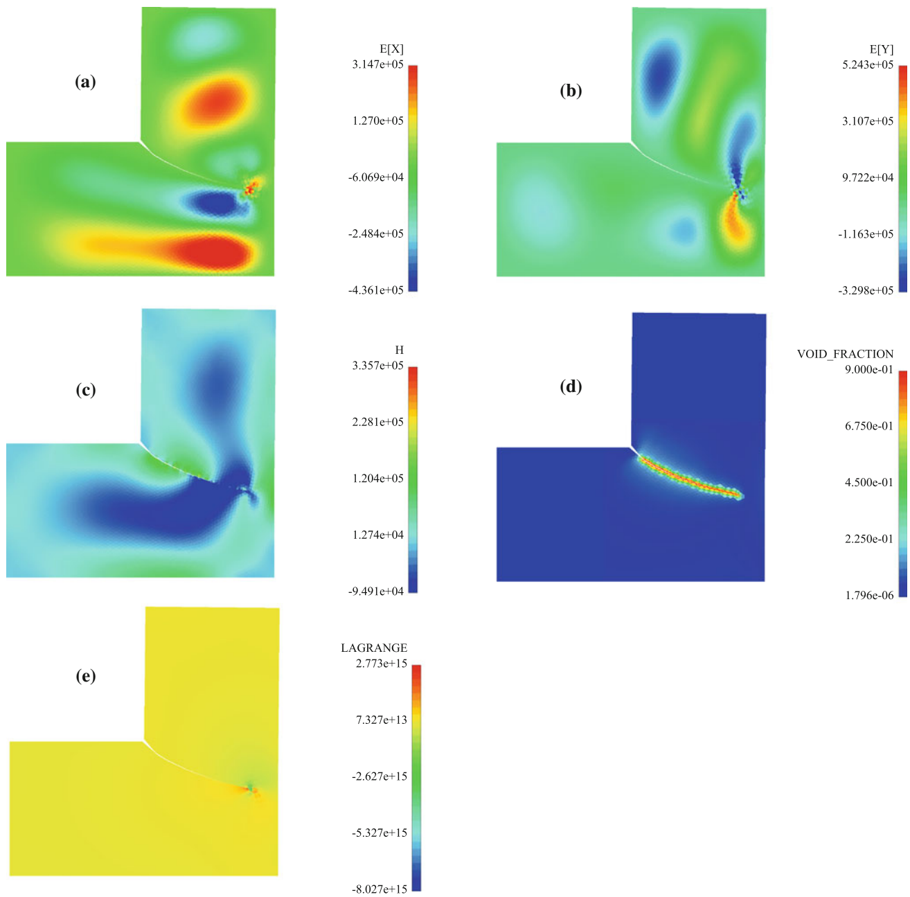
Fig. 10 Electric ( e ), magnetic ( h ), Lagrange multiplier ( \lambda ) and void fraction ( f ) fields for t = 4.175 \times 10^{-8} s. The mesh containing initially 11,824 elements is adopted. No displacement magnification is employed
