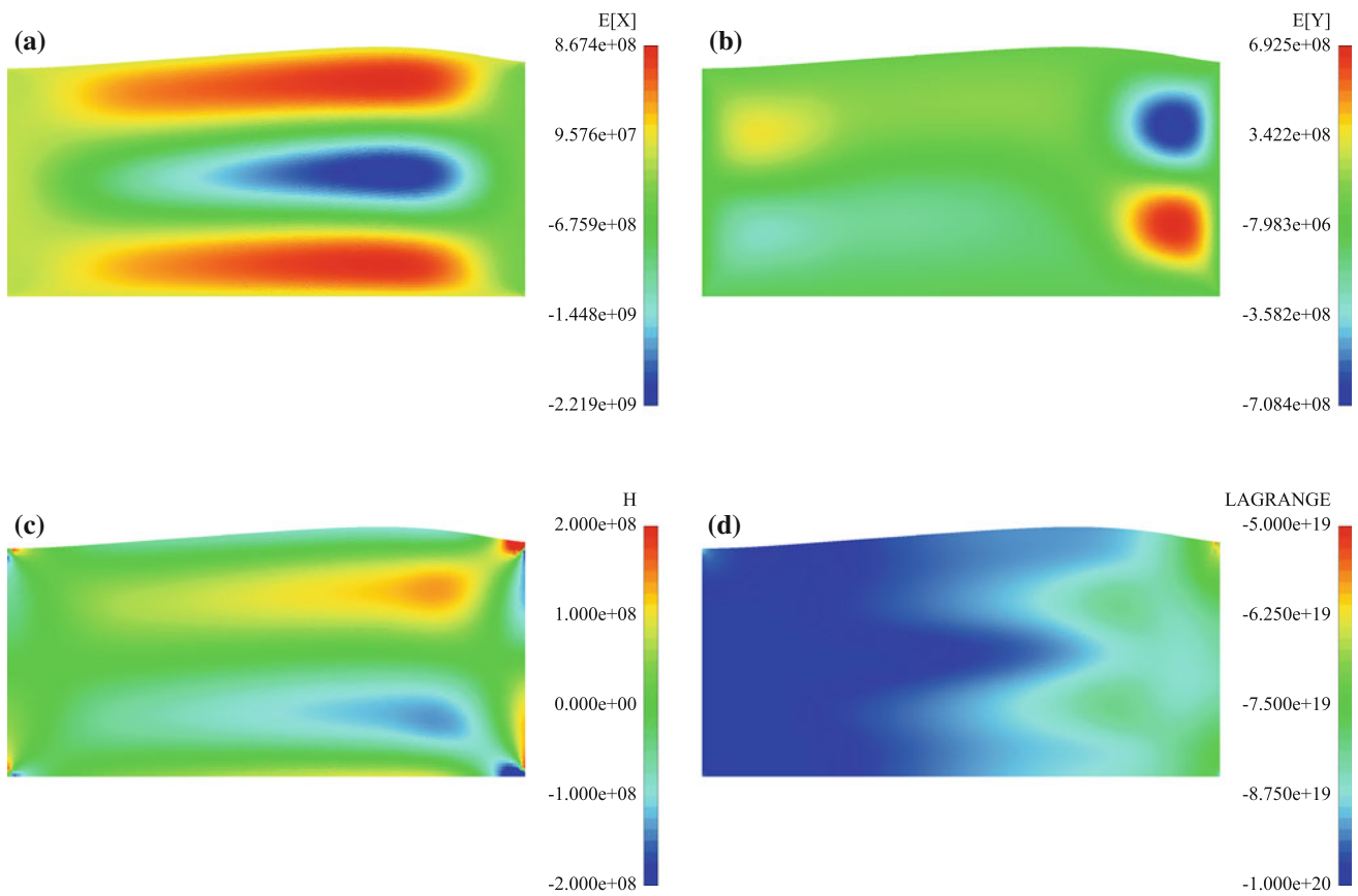
Fig. 6 Electric ( e ), magnetic ( h ) and Lagrange multiplier ( \lambda ) fields for t = 3.0 \times 10^{-8} s (not magnified)
