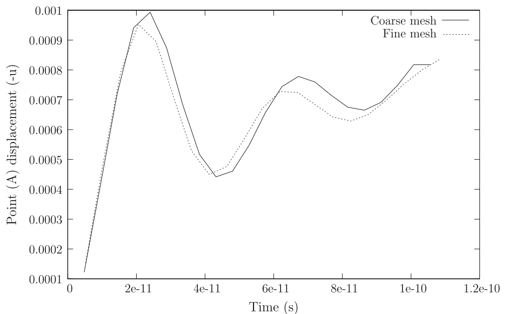
Fig. 5 Displacement/time results for point A for two mesh densities
