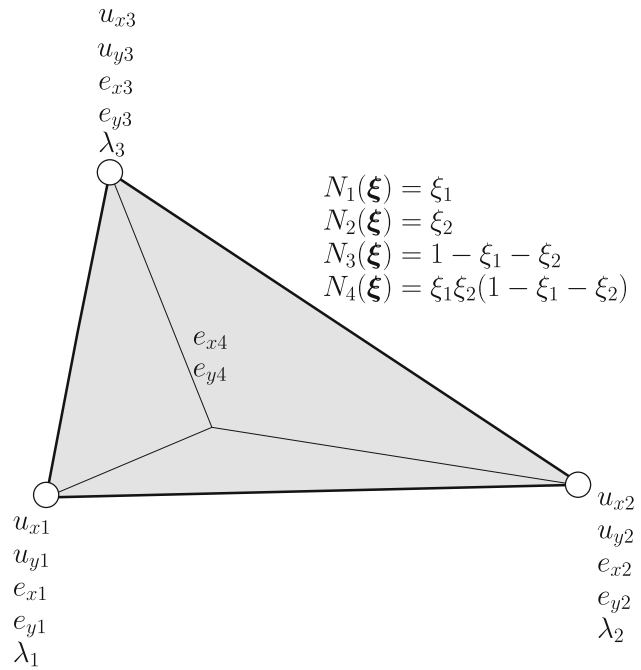
Fig. 3 Use of MINI element ([29]) for the mixed \boldsymbol{u} - \boldsymbol{e} - \boldsymbol{\lambda} problem
