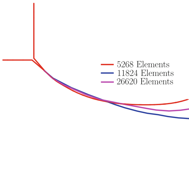
Fig. 9 Crack path comparison between the three meshes
