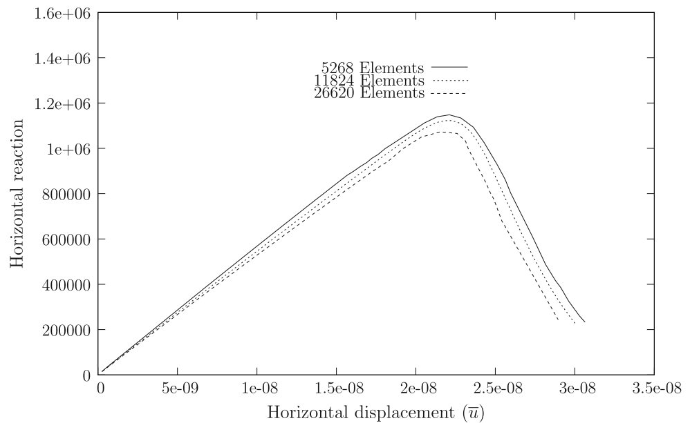
Fig. 8 Displacement/reaction results for the corner crack problem, comparing the three meshes. 1 m depth is considered
