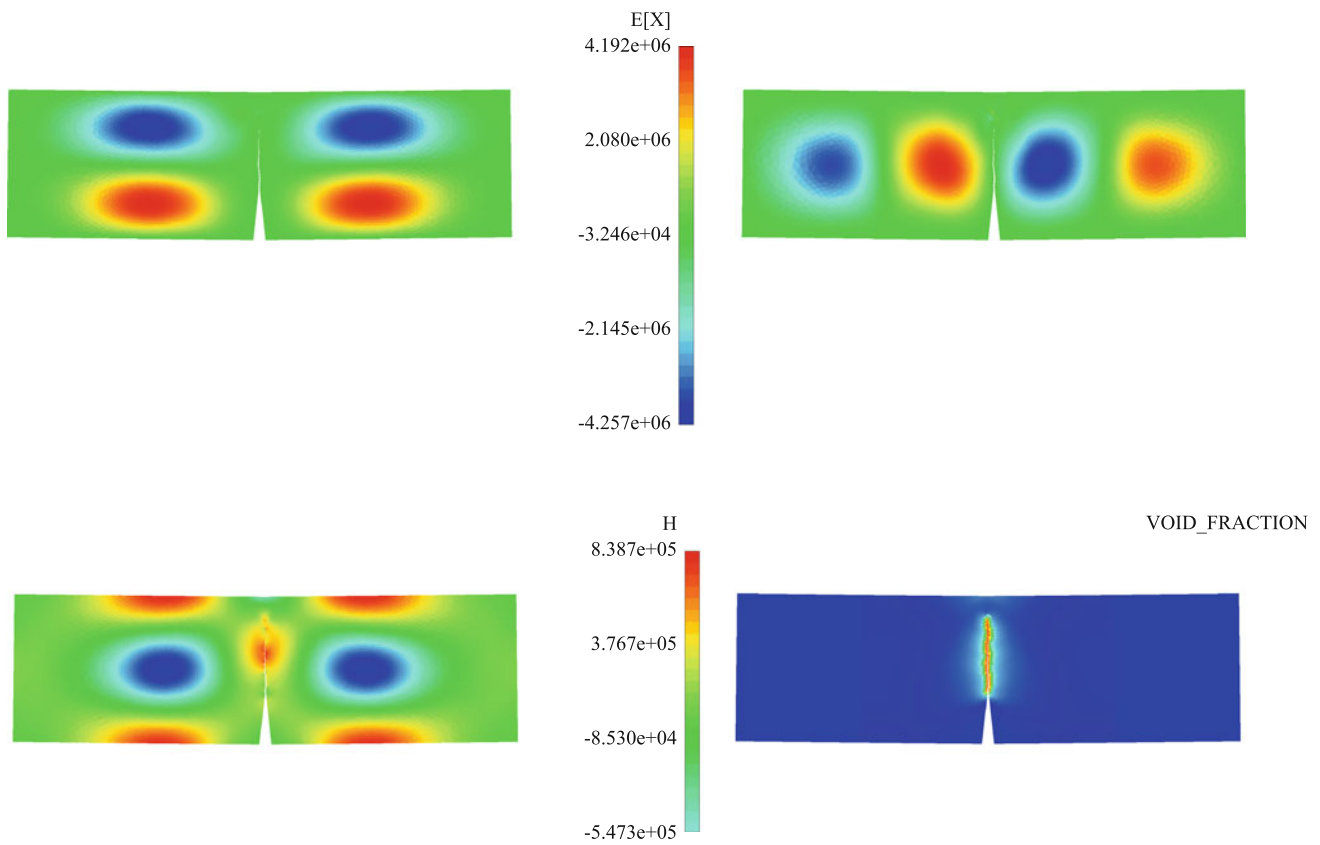
Fig. 13 Three-point bending test: electric ( e ), magnetic ( h ) and void fraction ( f ) fields for t = 8.38 \times 10^{-9} s and \alpha_{11} = 0
