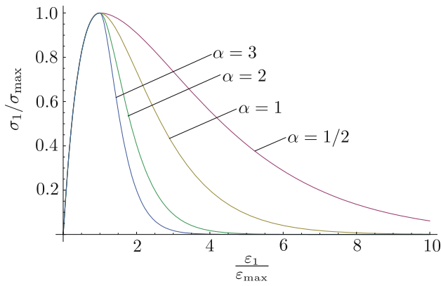
Fig. 2 One-dimensional representation of the damaged stress/strain relation
