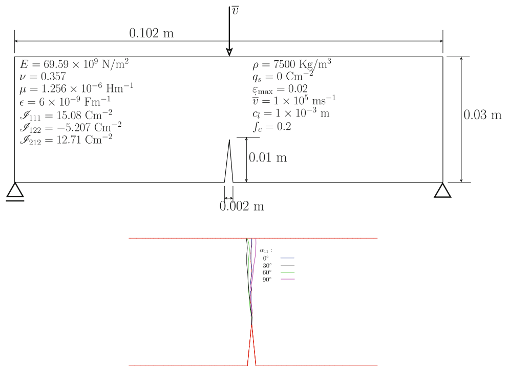
Fig. 11 Three-point bending test: relevant data and crack path results. A mesh with 6,585 nodes and with 12,858 triangles is employed
