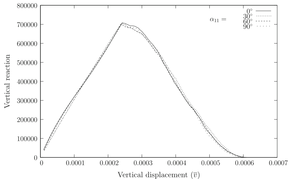
Fig. 12 Three-point bending test: vertical reaction as a function of \bar{v}
