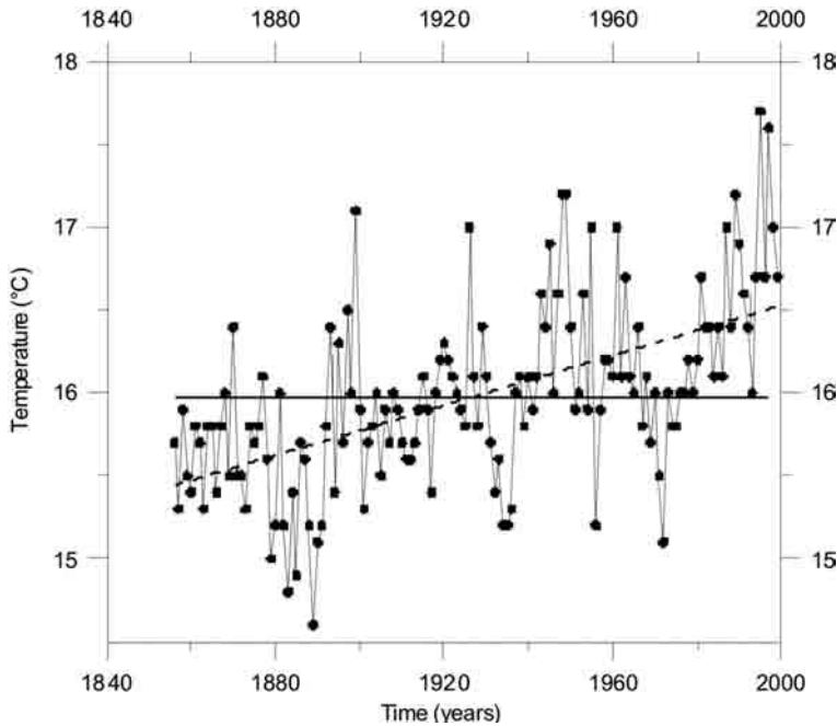
Fig. 4 – Air temperature time series for Lisbon weather station (dots). Also shown are the average temperature (solid line) and the linear fit to the to the temperature data (dashed line).
