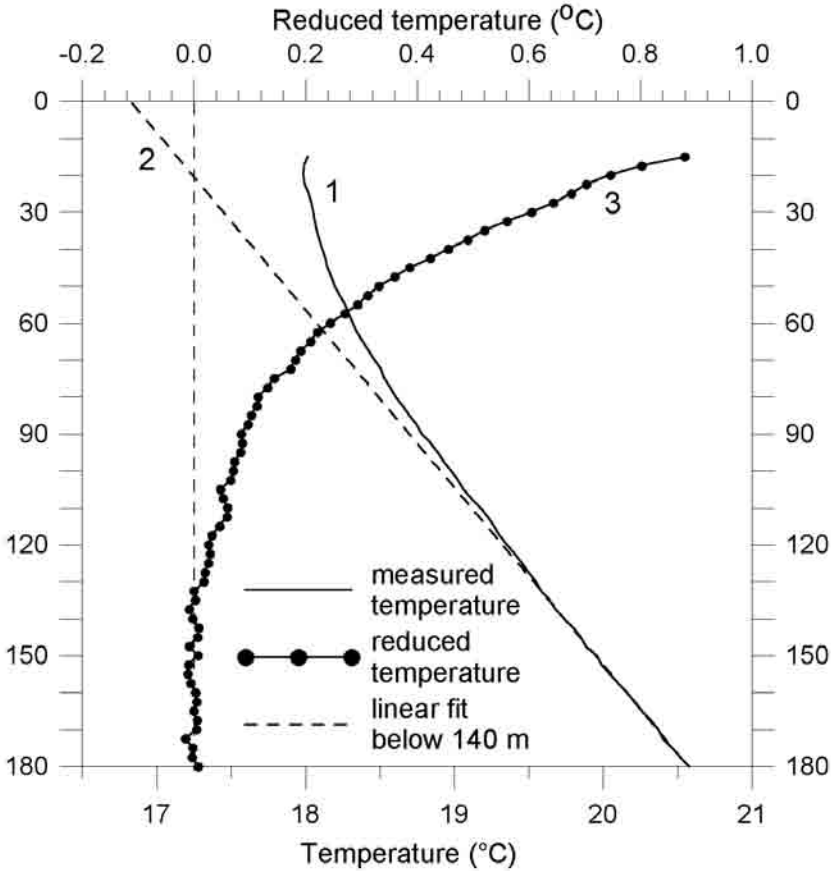
Fig. 2 – Temperature log obtained in 2003 in TGQC-1 borehole (line 1), as well as the steady-state component of the subsurface temperature (dashed line 2), and the reduced temperature (line 3), which is the difference between the actual temperature log and its steady-state component. Line 3 represents the climatic signal in TGQC-1 borehole.
