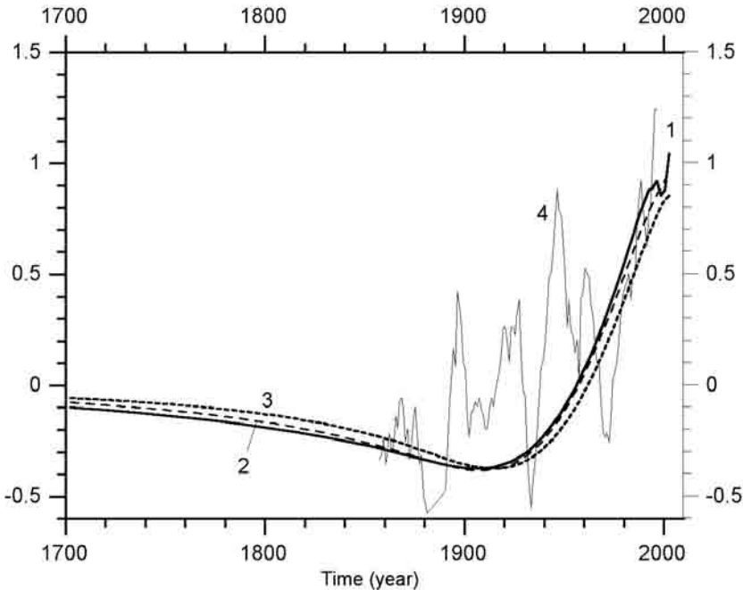
Fig. 3 – Ground surface temperature reconstructions obtained by applying the FSI method to the transient component of the temperature log obtained in the TGQC-1 borehole, with different levels of noise (lines 1-3) and for the thermal parameters mentioned in the text.
