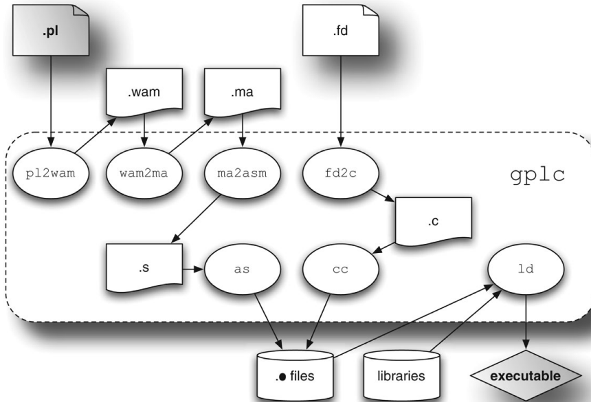
Fig. 1. Compilation scheme.
