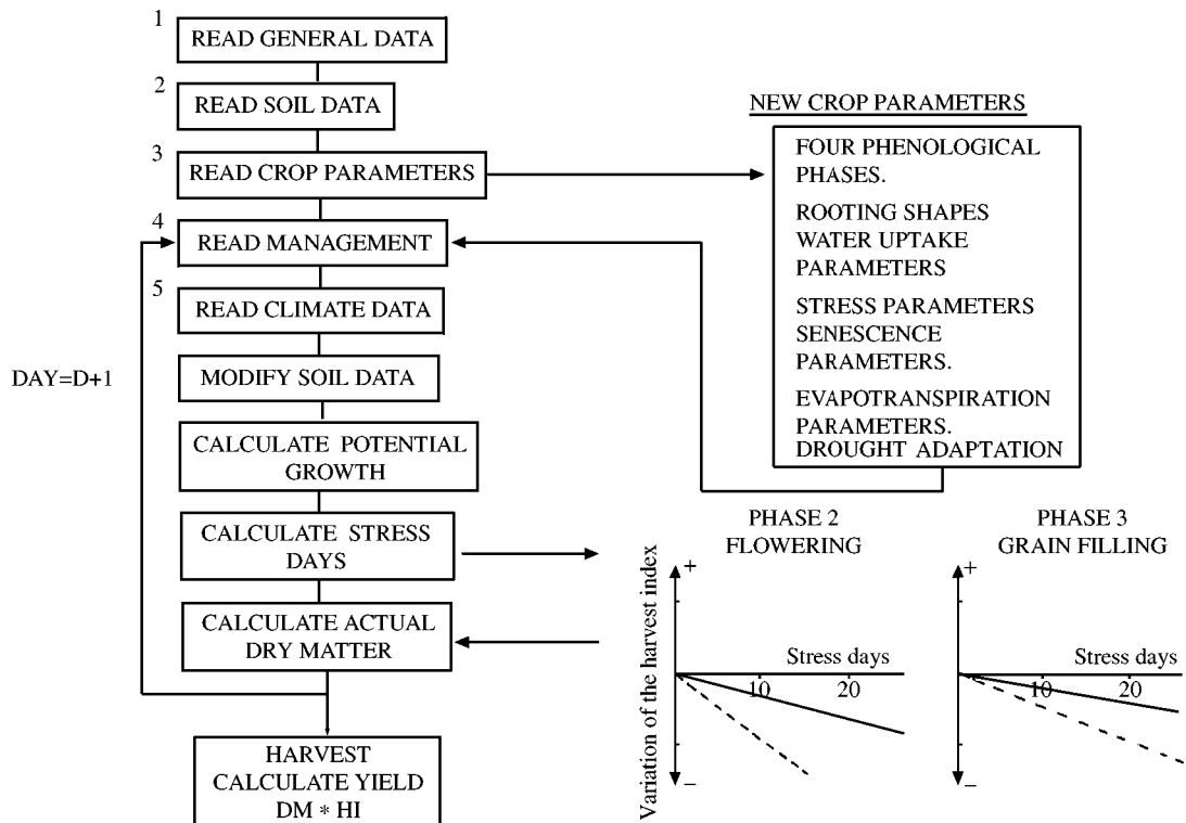
Fig. 1. Program flowchart for the erosion productivity impact calculator phase (EPIC-PHASE) model: DM, dry matter; HI, harvest index; —, effect on the harvest index of a moderate water stress; ----, effect of a high water stress
