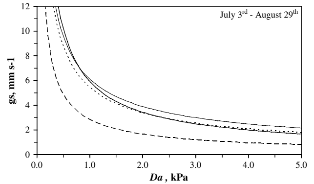
Fig. 6 – Best-fit relationship between stomatal conductance, g_s and air vapour pressure deficit, D_a from July 3rd to August 29th: —, treatment A; —, treatment B; · · ·, treatment C; - · -, dry-farming at the Herdade dos Lameirões site. D_a was determined for daylight hours (5:00–18:00 hour).
