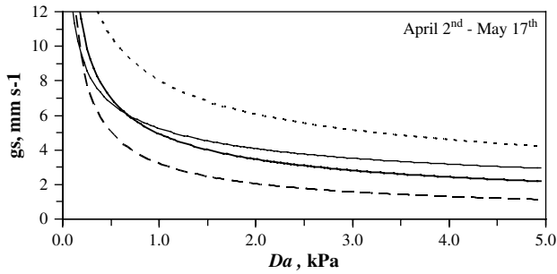
Fig. 4 – Best-fit relationship between stomatal conductance, g_s and air vapour pressure deficit, D_a from April 2nd to May 17th: —, treatment A; —, treatment B; · · ·, treatment C; - · -, dry-farming at the Herdade dos Lameirões site. D_a was determined for daylight hours (5:00–18:00 hour).
