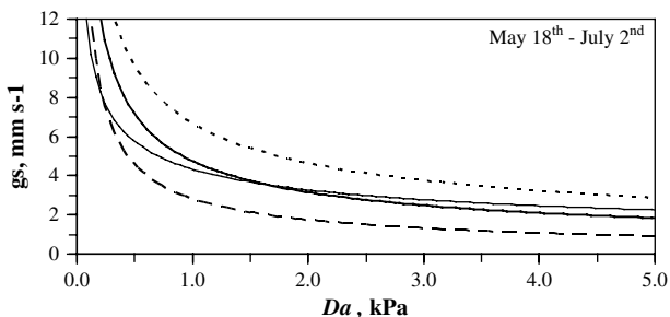
Fig. 5 – Best-fit relationship between stomatal conductance, g_s and air vapour pressure deficit, D_a from May 18th to July 2nd: —, treatment A; —, treatment B; · · ·, treatment C; - · -, dry-farming at the Herdade dos Lameirões site. D_a was determined for daylight hours (5:00–18:00 hour).
