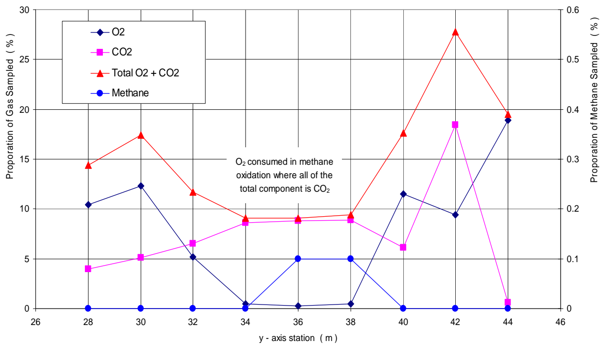
Fig. 2. Detection of methane in soil gas samples along x=32\text{m} - Grid C.
