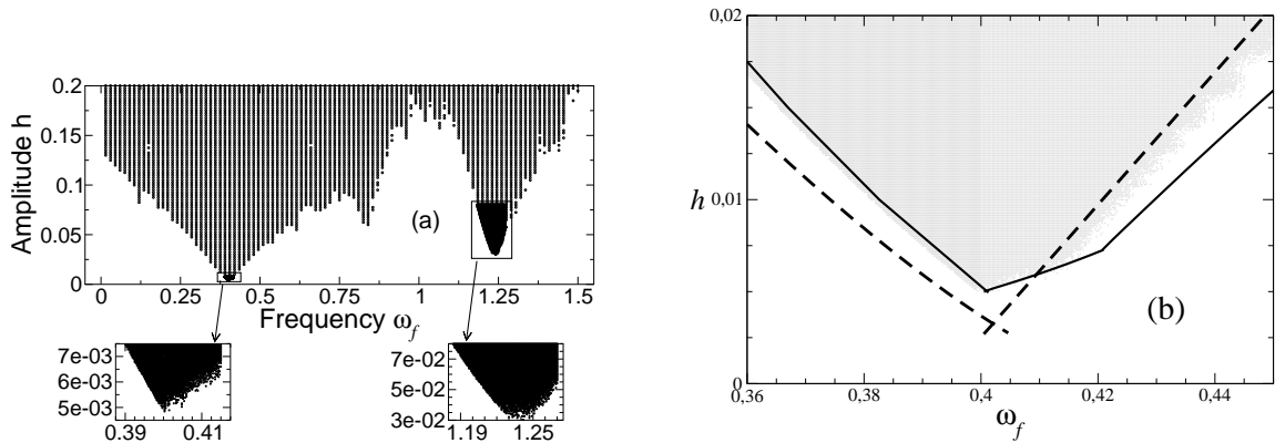
Fig. 6. (a) Bifurcation diagram for H = H_0 + hq \sin(\omega_f t) ; (b) the first minimum (shaded) and our theory: dashed line - the leading-order theory, solid line - the theory with higher-order corrections
