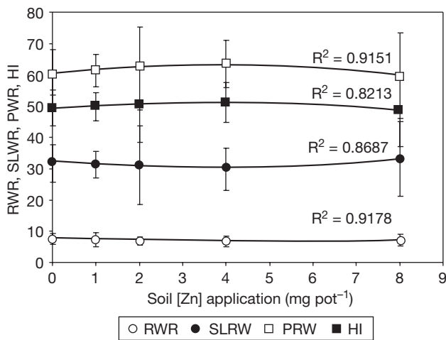
Figure 1. Relationships between soil Zn application and relative dry matter production of different organs of chickpea plants. RWR: roots weight ratio. SLWR: stems with leaves weight ratio. PWR: pot weight ratio. HI: harvest index. Represented points are treatment means.
