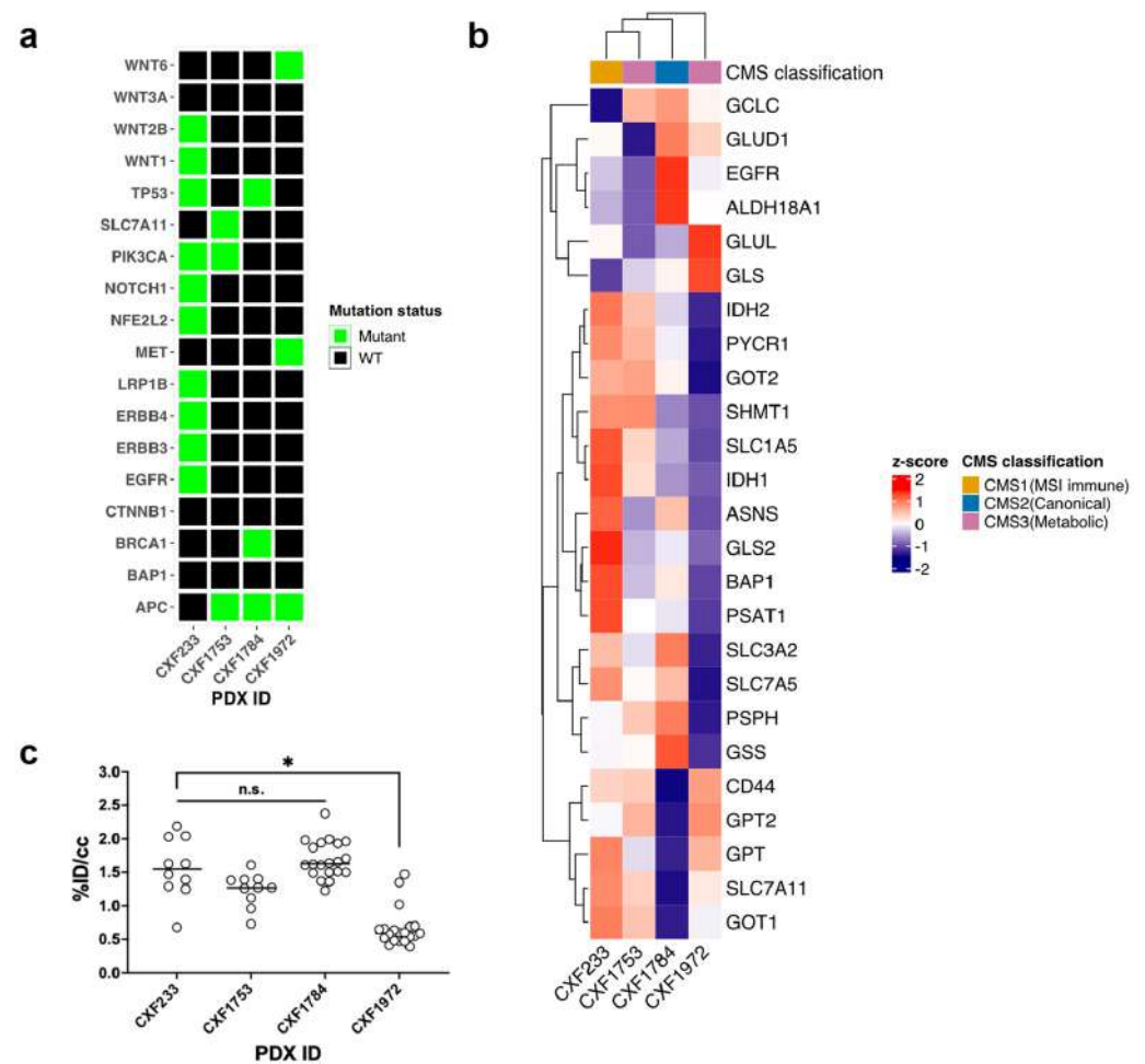
Figure 1. Baseline characteristics of wild-type (WT) KRAS colorectal cancer (CRC) patient-derived xenografts (PDXs). (a) Select mutational status highlighted in green for each PDX. (b) Transcriptomic profile with glutaminolysis-related genes. The consensus molecular subtype (CMS) was identified based on gene expressions of CRC. (c) Baseline (4S)-4-(3-[ 18 F]fluoro-propyl)-1-glutamate ([ 18 F]FSPG) uptake in PDX tumors. Each dot indicates [ 18 F]FSPG uptake in a PDX tumor of a mouse. [ 18 F]FSPG uptake as measured by the PET images were normalized to the injected dose and the mean radiotracer concentration within the volumes of interest (VOIs) drawn around the tumors. n.s.: “not significant”, *: p < 0.0001 .
