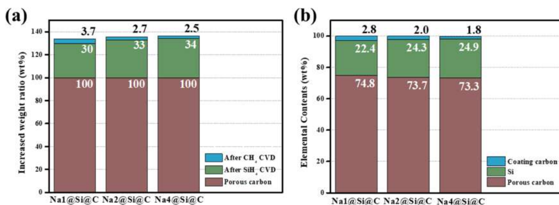
Figure 3. (a) Increased weight ratio of \text{Na}_x\text{@Si} and \text{Na}_x\text{@Si@C} after \text{SiH}_4 and \text{CH}_4 chemical vapor deposition (CVD). (b) Elemental contents of \text{Na}_x\text{@Si@C} .
