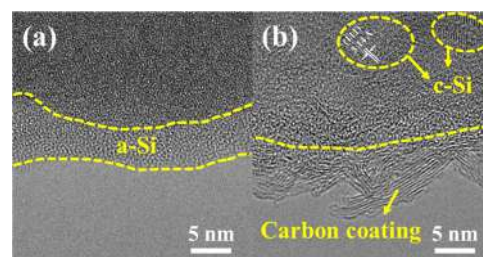
Figure 5. Transmission electron microscopy (TEM) images of (a) \text{Na}_2\text{@Si} and (b) \text{Na}_2\text{@Si@C} after \text{SiH}_4 and \text{CH}_4 CVD processes.
