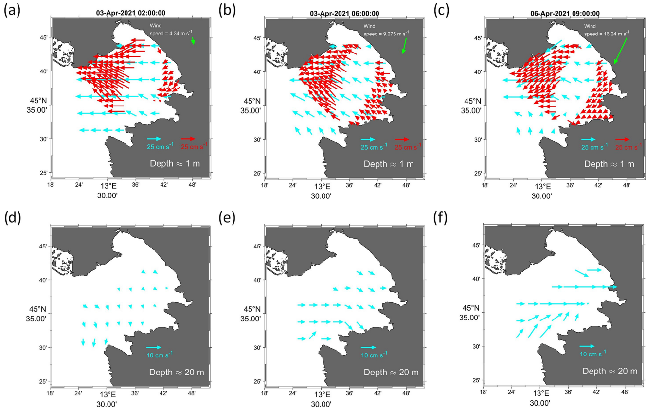
Figure 6. Maps of surface currents at \sim 1 m from the CMEMS model (blue arrows) and HFR (red arrows) on 3 April 2021 at 02:00 UTC (a) and 06:00 UTC (b), as well as on 6 April 2021 at 09:00 UTC (c). Maps of bottom currents at \sim 20 m from the CMEMS model (blue arrows) on 3 April 2021 at 02:00 UTC (d) and 06:00 UTC (e), as well as on 6 April 2021 at 09:00 UTC (f). Green arrows represent wind speed in metres per second ( \text{m s}^{-1} ).
