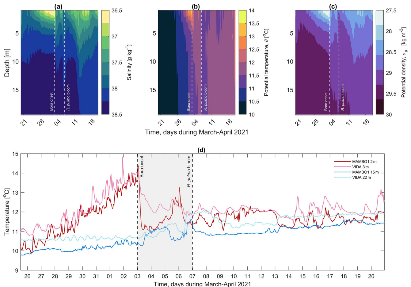
Figure 9. Hovmöller diagram of (a) salinity, (b) potential temperature and (c) potential density extracted from the CMEMS physical model for the period 20 March–20 April 2021. (d) Temperature time series recorded by the MAMBO1 buoy at 2 m (red line) and 15 m (blue line) and by the VIDA buoy at 3 m (pink line) and 22 m (light blue line).
