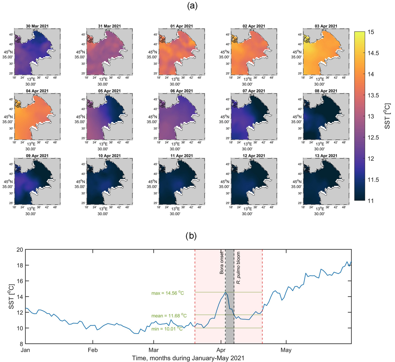
Figure 8. (a) Maps of daily SST showing the evolution of the surface temperature field and the effect of the bora wind in the GOT from 30 March to 13 April 2021. Here the colour bar represents the SST field in degrees Celsius ( ^{\circ}\text{C} ). (b) Time series of the aforementioned dataset spatially averaged over the extracted area for the period 1 January to 30 May 2021. The shaded grey area represents the bora–bloom period, with the left black dashed line delimiting the start of the bora episode and the right black dashed line representing the day when the jellyfish bloom was reported by the media and citizens. The shaded red are between the dashed vertical red lines delimits the interval 20 March–20 April 2021, and the green lines represent the max, mean and min values during this interval.
