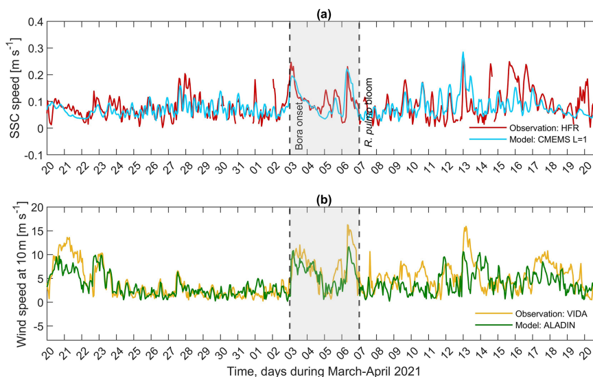
Figure 5. Times series of hourly (a) sea surface current (SSC) speed from the CMEMS physical model (blue line) and HF radar (red line) spatially averaged over the extracted area. (b) Wind speed from the ALADIN atmospheric model (green line) and VIDA buoy (orange line) extracted at 13.55° E, 45.55° N and 13.55° E, 45.63° N, respectively, from 20 March to 20 April 2021. The shaded area represents the bora-bloom period, with the left dashed black line delimiting the start of the bora episode and the right dashed black line representing the day when the jellyfish bloom was reported by the media and citizens.
