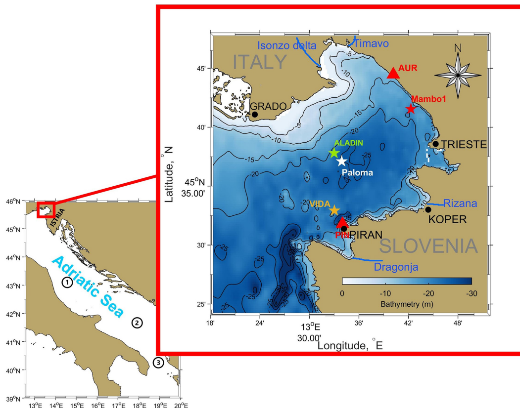
Figure 2. R. pulmo Adriatic Sea coastline map and Gulf of Trieste bathymetry (GOT, red box) with locations where the multi-platform data were extracted. The colour bar represents the GOT bathymetry, as do the contour lines. Blue lines represent the main rivers influencing the area. The green star indicates the locations where ALADIN model wind data were extracted, while the orange star shows the VIDA buoy position. The white star represents the location of the Paloma site where CTD ship measurements were taken. Red triangles represent the location of high-frequency radar stations, and the red star indicates the position of the MAMBO1 buoy. Numbers represent the following: 1, Jabuka or middle Adriatic pit; 2, southern Adriatic pit; 3, Strait of Otranto.
