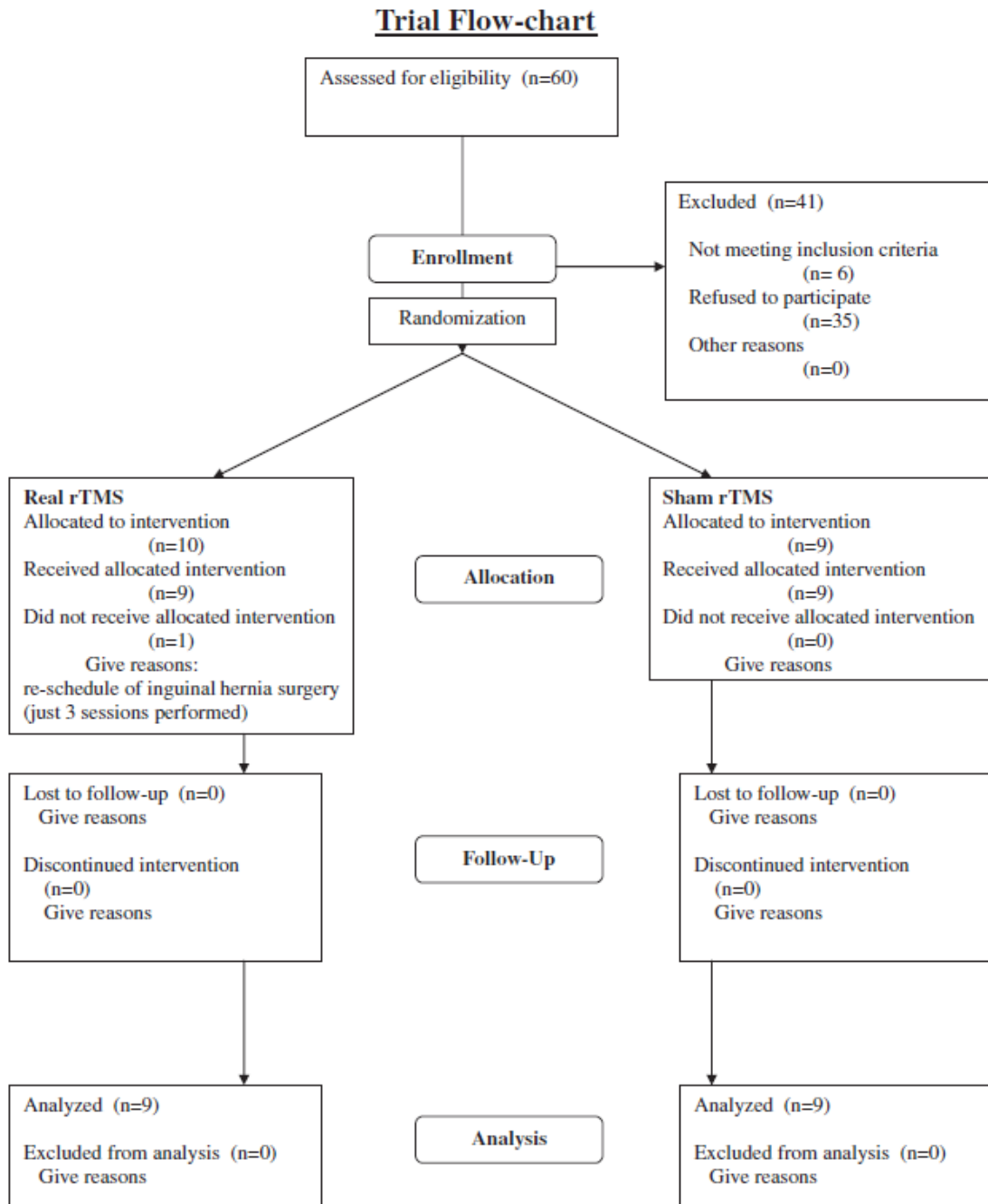
Fig. 1. Trial flow-chart.
