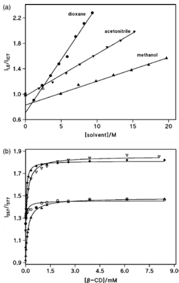
Figure 6 Plot of the ratio I_{LE}/I_{ICT} as a function of (a) solvent concentration in the aqueous mixture dioxane ( \bullet ), AN ( \blacktriangledown ), MeOH ( \blacktriangle ); (b) \beta -CD concentration in strong acid, HCl ( \blacktriangle ); mild acid, acetic acid–acetate ( \circ ); mild base, carbonate–bicarbonate ( \blacktriangledown ), and alkaline medium ( \blacklozenge ).
