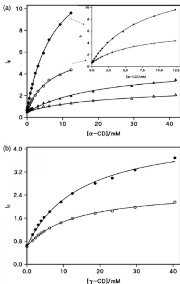
Figure 5 Variation of the fluorescence emission intensities of 10.4 \mu M TCA dissolved in water (a) at 0.033 M carbonate–bicarbonate (1:1) buffer ( \circ, \bullet ) and at 0.067 M acetic acid–acetate (1:1) as a function of \alpha -CD concentration ( \blacktriangledown, \blacktriangledown ); the inset shows the indicated expanded plot, and (b) at 0.033 M carbonate–bicarbonate (1:1) buffer ( \circ, \bullet ), as a function of \gamma -CD concentration; (open) symbols correspond to 377 nm or ICT emission state, (solid) symbols correspond to 357 nm or LE emission state.
