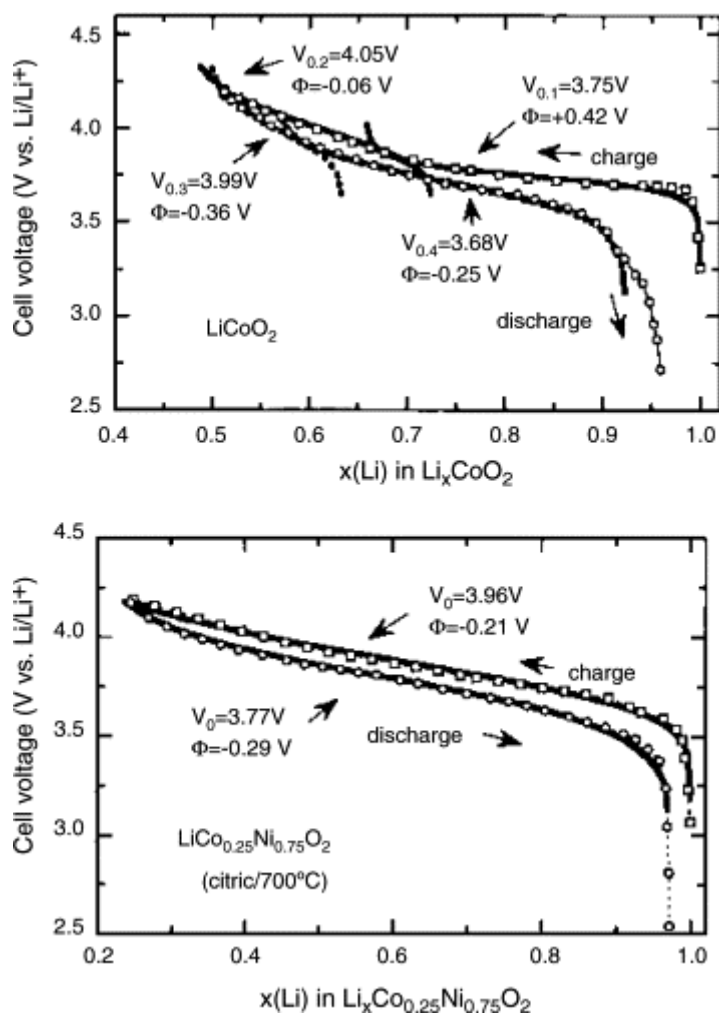
Fig. 14. Typical fits of the charge–discharge for \text{Li}||\text{LiCoO}_2 and \text{Li}||\text{LiCo}_{0.25}\text{Ni}_{0.75}\text{O}_2 cell profiles using Eq. (4) showing the single-phase and two-phase regions. Dashed and full lines represent the experimental and calculated voltage–composition curves, respectively.
