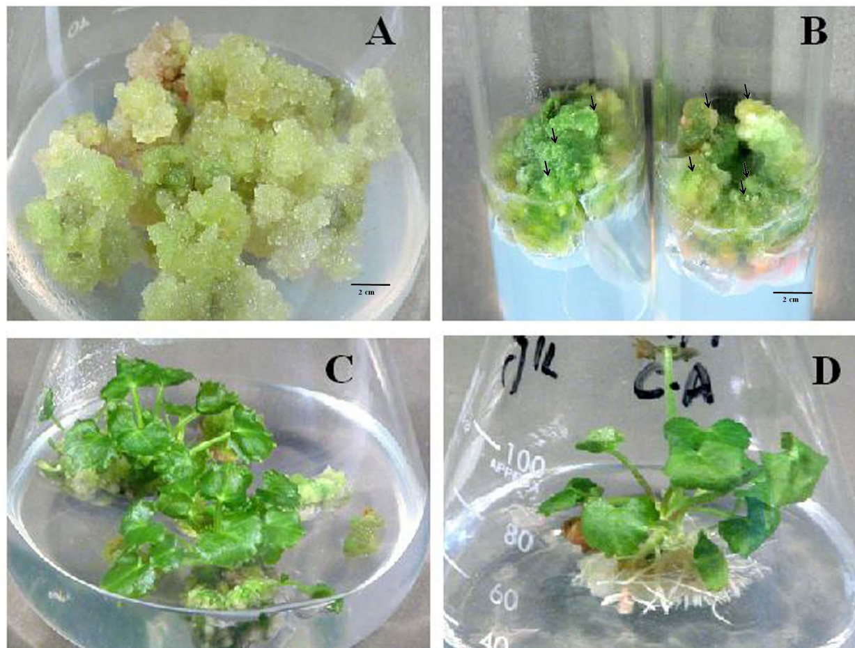
Figure 1 Callus formation and organogenesis of Centella asiatica L. from leaf explant on MS media containing; (A) callus formation on 5.37 \mu\text{M} NAA+2.21 \mu\text{M} BA; (B) callus formation on 5.37 \mu\text{M} NAA+4.42 \mu\text{M} BA; (C) shooting at 4.42 \mu\text{M} BA+5.37 \mu\text{M} NAA; (D) rooting at 10.74 \mu\text{M} NAA.
