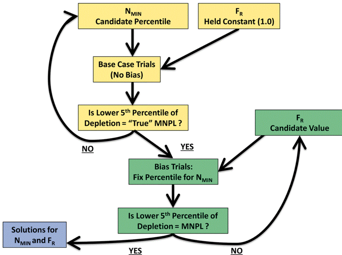
Figure 1: Flow diagram of Wade’s (1998) procedure for solving for values of N_{min} and F_R that meet the MMPA CO (taken from Brandon et al. 2017, © International Council for the Exploration of the Sea 2016). Note that the ASCOBANS CO is different from the MMPA CO and this new values of N_{min} and F_R need to be determined.
