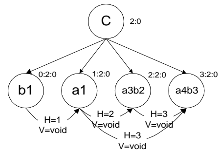
Figure 6 - New case
