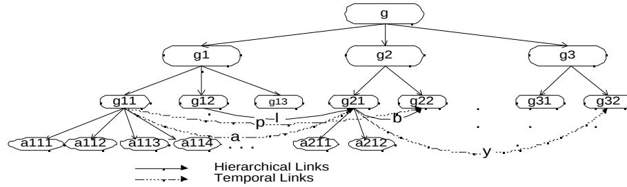
Figure 1 - Case structure. The g_i 's represent the goals and the a_i 's the actions.
