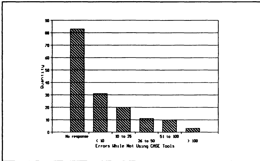
Figure H-12. Requirements Analysis Errors/KLOC of All Surveyed Organizations Not Using CASE Tools
