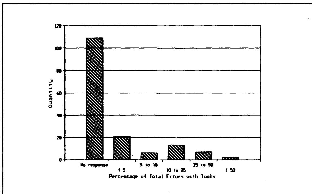
Figure H-15. Percentage of Total Errors Credited to Requirements Analysis in All Surveyed Organizations Using CASE Tools
