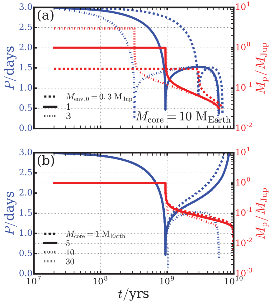
Fig. 7 Mass (red lines) and orbital (blue lines) evolution for hot Jupiter systems with initial periods P_0 = 3 days and Q_* = 10^5 and a variety of initial envelope masses M_{env,0} and core masses M_{core} . The different linestyles indicate different planetary parameters. (a) Hot Jupiters with M_{env,0} = 0.3, 1, 3 M_{Jup} and M_{core} fixed at 10 M_{Earth} . (b) Hot Jupiters with M_{env,0} = 1 M_{Jup} and M_{core} = 1, 5, 10, 30 M_{Earth} . These calculations assume \delta\gamma = 0.5 , i.e. half the orbital angular momentum carried by the escaping gas is lost.
