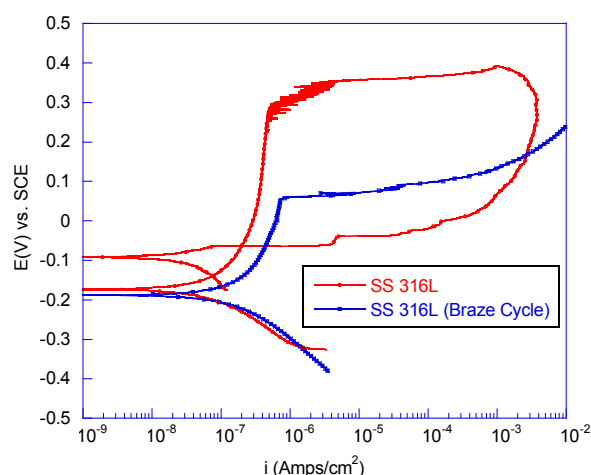
Figure 6. Potentiodynamic polarization scans conducted on 316L stainless steel subjected to a thermal brazing cycle (blue curve) compared to unfired 316L (red curve). Testing was conducted in 0.6 M NaCl with a scan rate 0.166 mV/s.
