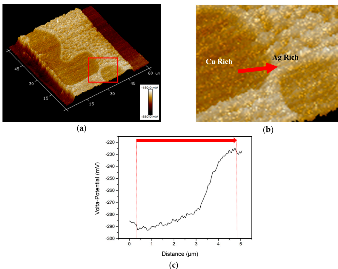
Figure 11. (a) Three dimensional (3-D) SKPFM Volta potential image of Cu-Ag-Ti sample with a box indicating area of scan; (b) Zoomed in image with arrow indicating where scan was taken; and (c) Graph of potential values obtained from scan as a function of distance with indicating arrow.
