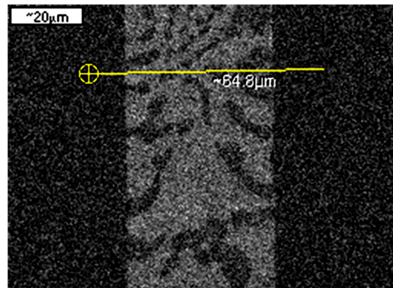
Figure 2. (a) SEM micrograph and (b) energy dispersive spectroscopy (EDS) line scan results from the cross section of a 316L stainless steel/Cu-Ag-Ti brazed joint.
