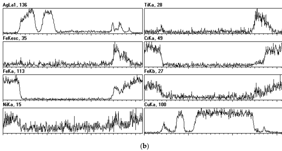
Figure 2. (a) SEM micrograph and (b) energy dispersive spectroscopy (EDS) line scan results from the cross section of a 316L stainless steel/Cu-Ag-Ti brazed joint.
