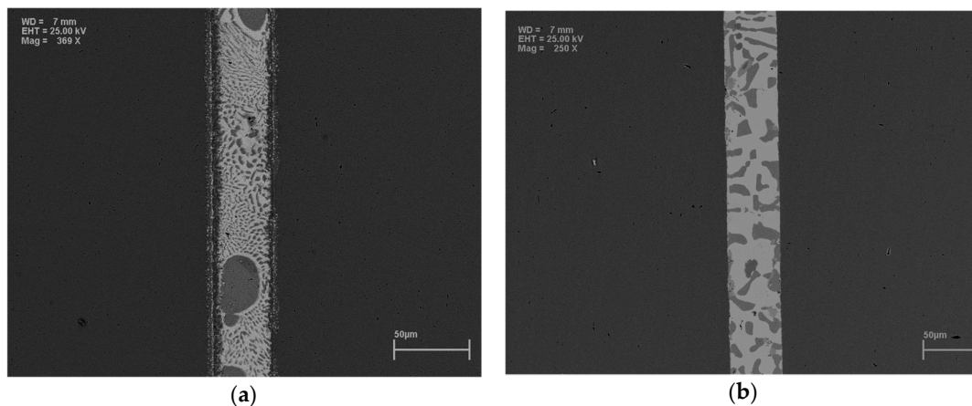
Figure 1. Scanning Electron Microscopy (SEM) images of cross sections of the resultant braze joint between two stainless steel 316L samples joined using: Cu-Ag-Ti (a) and Cu-Ag-In-Ti (b) braze alloys.
