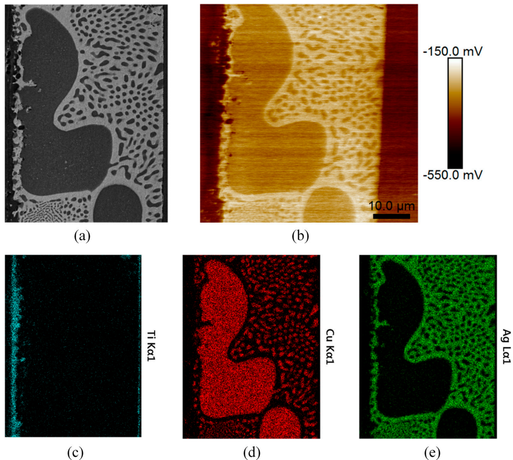
Figure 8. Secondary electron SEM image of Cu-Ag-Ti sample (a) followed by corresponding Scanning Kelvin Probe Force Microscopy (SKPFM) surface potential image (b). EDS elemental maps of the identical region for: Titanium (c); Copper (d); and Silver (e) are shown.
