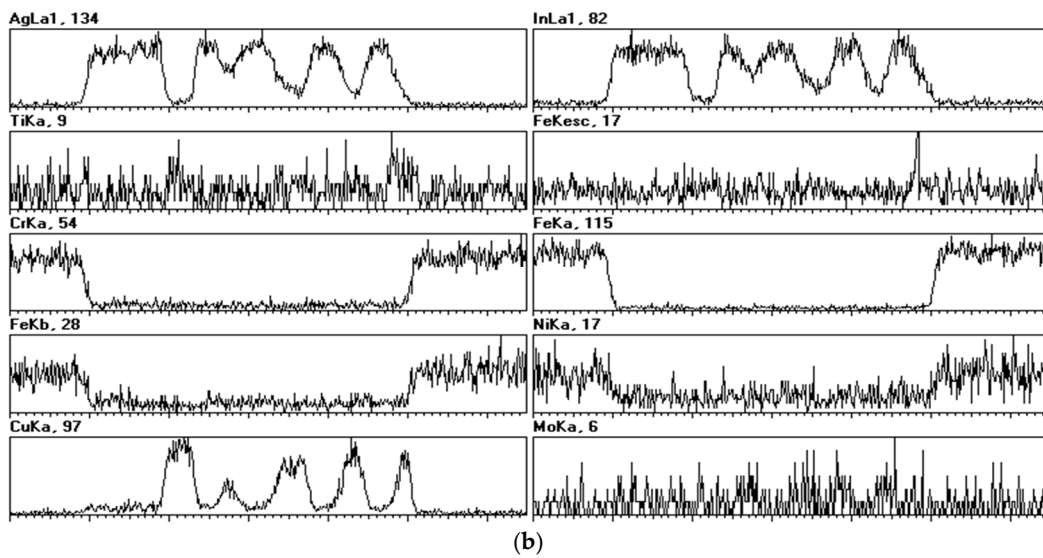
Figure 3. (a) SEM micrograph and (b) EDS line scans of a cross section of a 316L stainless steel/Cu-Ag-In-Ti brazed joint.
