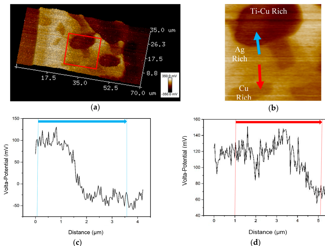
Figure 12. (a) 3-D SKPFM potential image of Cu-Ag-In-Ti sample with a box indicating area of scan. (b) Zoomed in image with arrows indicating where scan was taken. Graph of potential values obtained from scan as a function of distance with indicating arrow: (c) Blue arrow (Ag-rich phase to Ti-Cu-rich phase); and (d) Red arrow (Ag-rich phase to Cu-rich phase).
