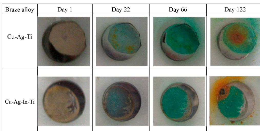
Figure 7. Time lapse photographs of corrosion propagation during long term exposure testing in 0.6 M NaCl. Cu-Ag-Ti (top) and Cu-Ag-In-Ti (bottom) braze alloy foil disks were used to coat ~80% of the exposed face area on 316L stainless steel samples. The stainless steel disk diameter was 16 mm for both samples.
