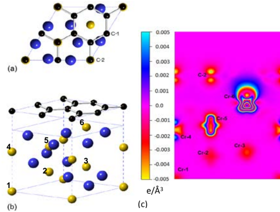
Fig. 2. Atomic structure and charge density of graphene- \text{Cr}_2\text{O}_3 : (a) top and (b) side view of used supercell, and (c) charge density difference with isovalues from -0.005 to 0.005 e/\text{\AA}^3 . Cr, O and C atoms are shown in yellow, blue and black colors. C-1 and C-2 are the carbon atoms near to and away from the top-Cr atom, respectively. The films are separated by a supercell vacuum of 18 \text{\AA} .
