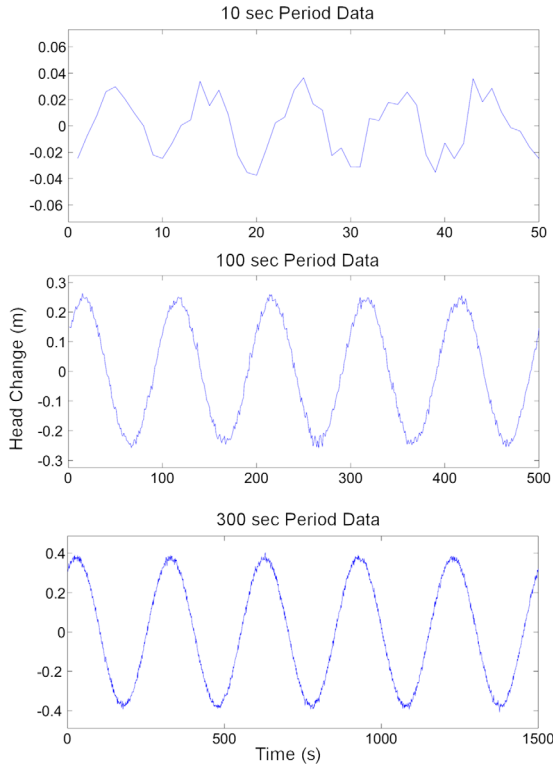
Figure 9. Examples of raw data used in inversions. Figure shows noisy records from North observation well at three different stimulation periods (10, 100, and 300 s periods).
