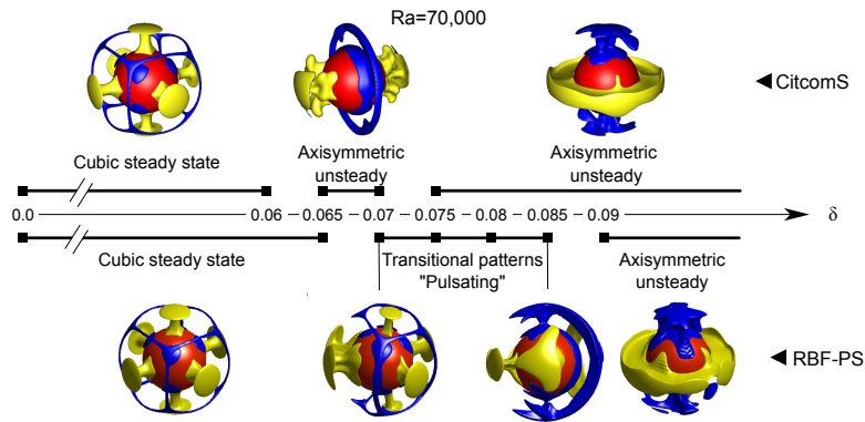
Fig. 4. Stability of the cubic steady state at Ra = 70\,000 with CitcomS (up row) and the RBF-PS method (bottom row). The cubic steady state pattern is destabilized for \delta \geq 0.065 with CitcomS and \delta \geq 0.07 with RBF-PS. The figure highlights transitional patterns between the two main geometries.
