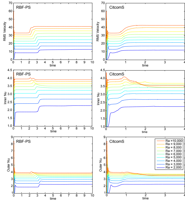
Fig. 10. Transition between steady states, as evidenced by both the RBF-PS and CitComS models, in the (V_{rms}) (top panels), Nu_i (middle panels), and Nu_o (bottom panels) for the dodecahedral initial condition.
