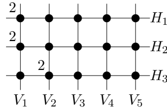
FIGURE 2.4.2. A configuration where greedy choices are not optimal.
