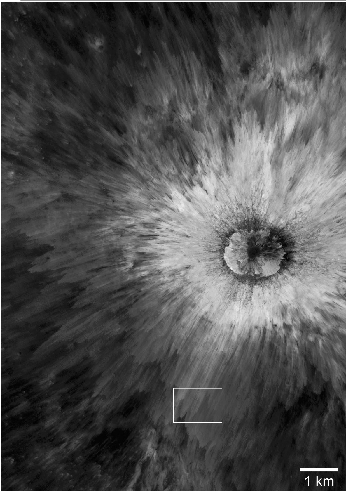
Figure 7. Mosaic of LROC images M110601418L/R and M125936995L/R centered near 151.7°E, 4.1°S. This image shows the proximal layered ejecta deposits with their continuous, striated character. As shown in Figure 3, cold spot surfaces are further away from the crater than these deposits. The white box denotes the area of detail shown in Figure 3.
