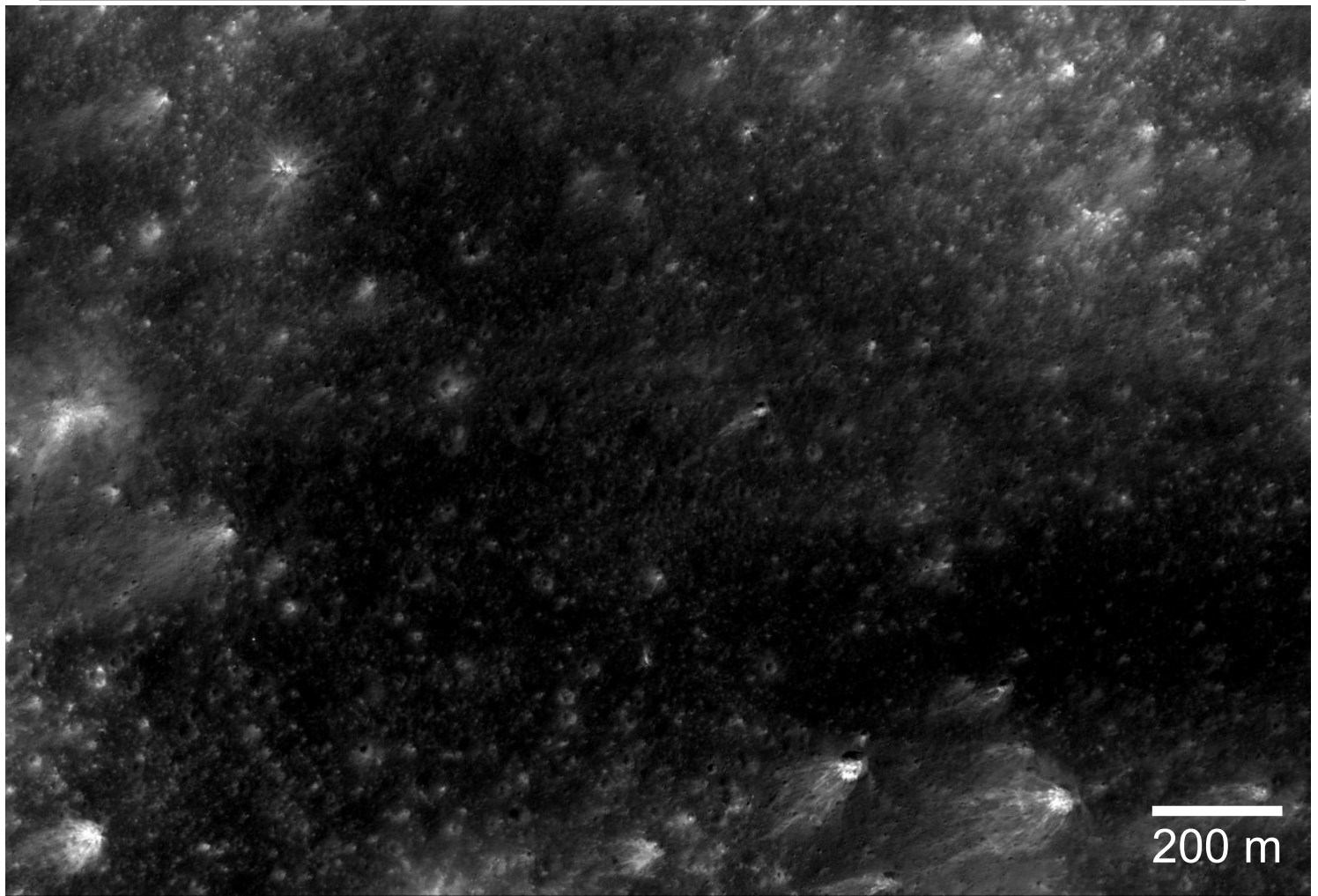
Figure 12. LROC image (M123581454R; Solar incidence 12^\circ ) covering a cold spot surface near 151.0^\circ\text{E} , 4.2^\circ\text{S} . Relatively bright, wispy surfaces trail away from the nearby source crater behind topographic features. However, the most prominent cold temperature anomalies coincide with relatively dark featureless surfaces within the image shown.
