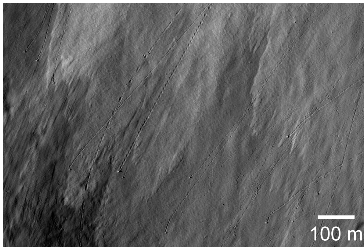
Figure 8. LROC Images M11060141R (top; Solar incidence 17^\circ ) and M118858378R; Solar incidence 66^\circ ). Both images cover the same location denoted by the white box shown in Figure 7. High angles of solar incidence illustrate the surface textural characteristics and low angles of solar incidence show the albedo characteristics of the proximal layered ejecta deposits.
