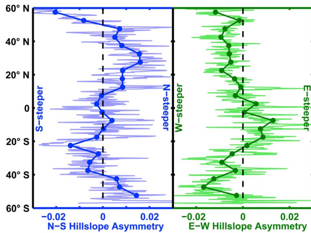
Figure 2. Average HA values within 5^\circ (darker lines) and 0.25^\circ (lighter lines) latitude-bins for the American Cordillera. Both N–S and E–W HA display gradual trends and reversals in sign with latitude, suggesting latitude-based influences.
