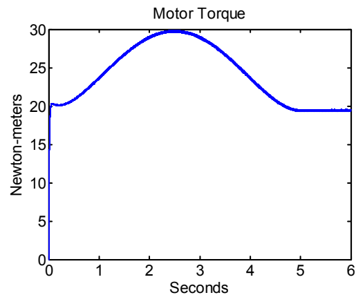
Fig. 8. Torque using proposed multilevel inverter.
