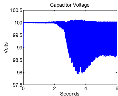
Fig. 9. Capacitor voltage versus time.
