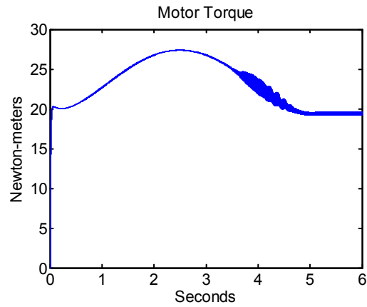
Fig. 7. Torque using standard 3-leg inverter.
