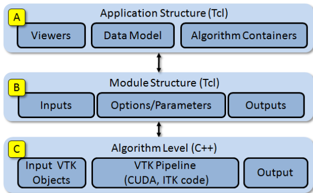
Fig. 4 BioImage Suite Architecture. Main Application Structure (A), Module Structure (B) and Algorithm level data processing (C++ Implementation) (C). All parts of A+B are written in Incr Tcl and invoke C++ code wrapped with a TCL access layer as pioneered by VTK.
