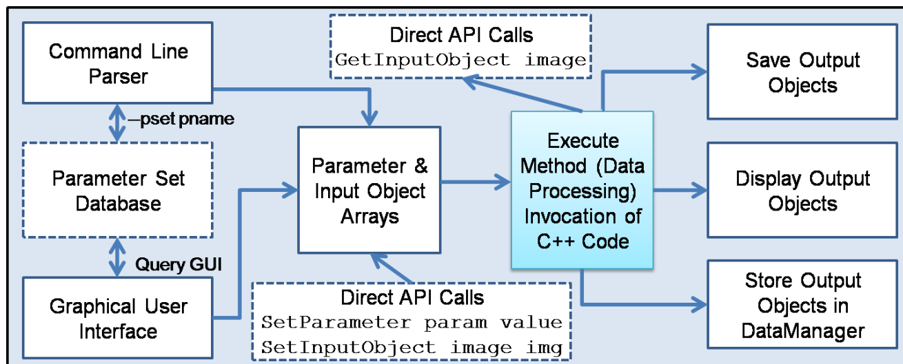
Fig. 8 BioImage Suite Module Architecture – detail view of Fig. 4B: the structure of a Module. The inputs and parameters can be specified in three ways: (i) command line, (ii) GUI, (iii) direct application programming interface (API) calls. Then the exact same Execute method is invoked and the outputs stored/displayed as appropriate.
