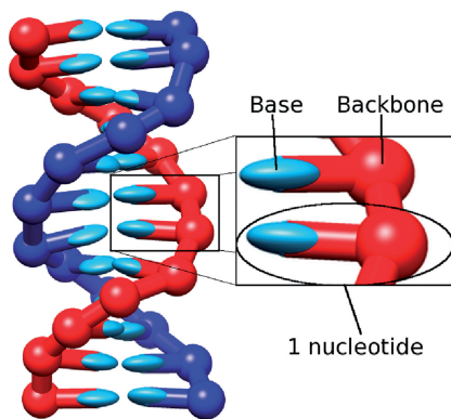
Figure 9. A 12-bp DNA duplex as represented by oxDNA. The enlarged section shows two rigid nucleotides, highlighting the backbone and base parts. The planarity of bases is captured through the orientational dependence of interactions. Image reproduced from Ouldridge et al. [90].
