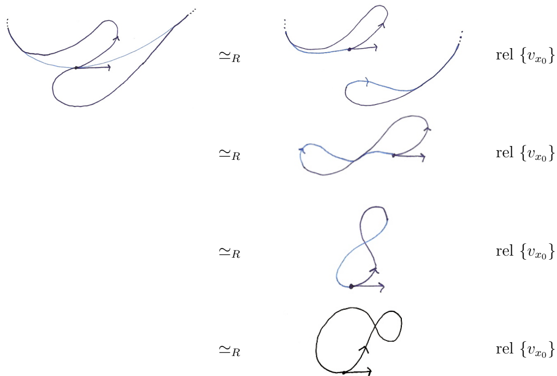
Figure 2.8: Regular homotopy showing \left[ (\gamma \circ r) \cdot (((\bar{f} \circ r) \cdot (\delta \circ r)) \circ r) \right]_R \cdot [f]_R = [e]_R .
