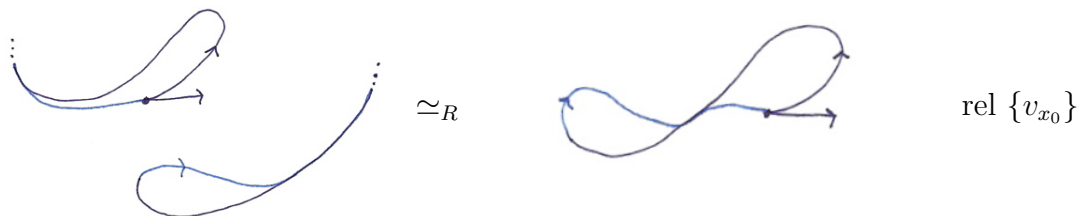
Figure 2.9: Regular homotopy from Figure 2.8.
