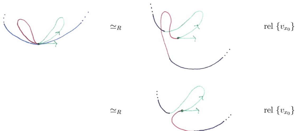
Figure 2.7: A regular homotopy of (\gamma \circ r) \cdot (((\bar{f} \circ r) \cdot (\delta \circ r)) \circ r) .
