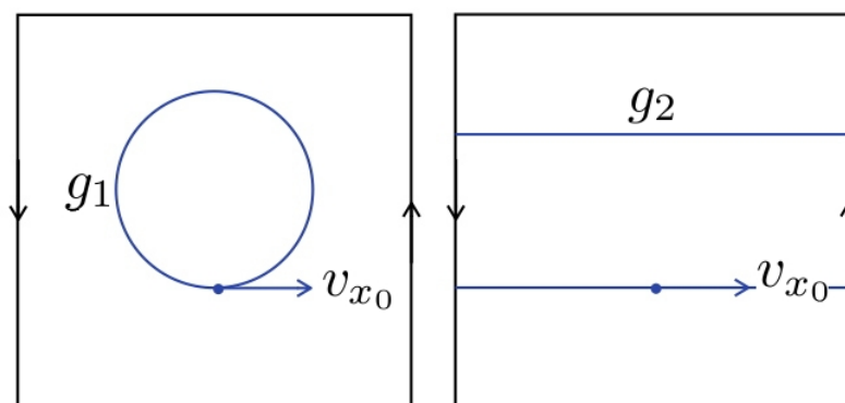
Figure 4.4: [g_1]_R and [g_2]_R generate \pi_R^{or}(B, v_{x_0}) .
