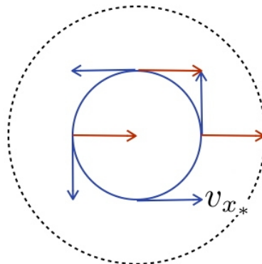
Figure 3.2: a_1 pictured with vectors Y_{a'_1}(t) and Y_{\widehat{X}_{a_1}}(t) for four values of t .
