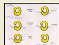
Figure 2: Topoisomerase cutting and rejoining DNA strands
