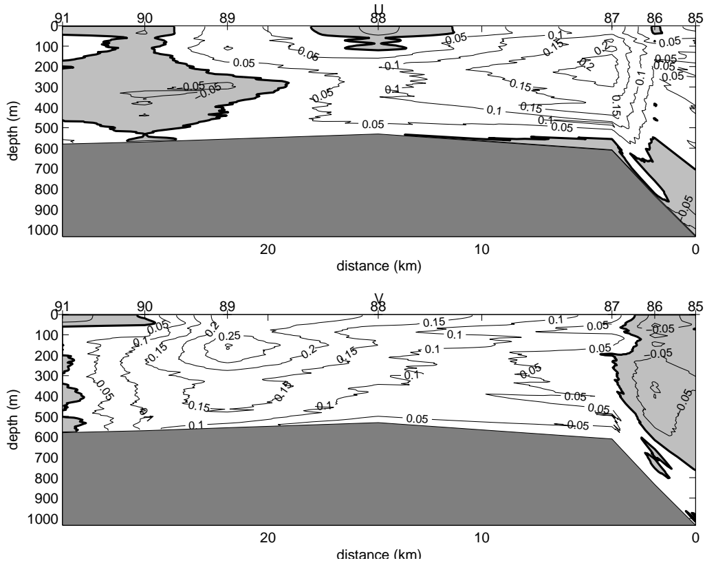
Fig. 23. Contour plot of LADCP velocities (in m/s) on section 8. Shaded areas represent negative values of u or v . The contour for 0 is bold.
