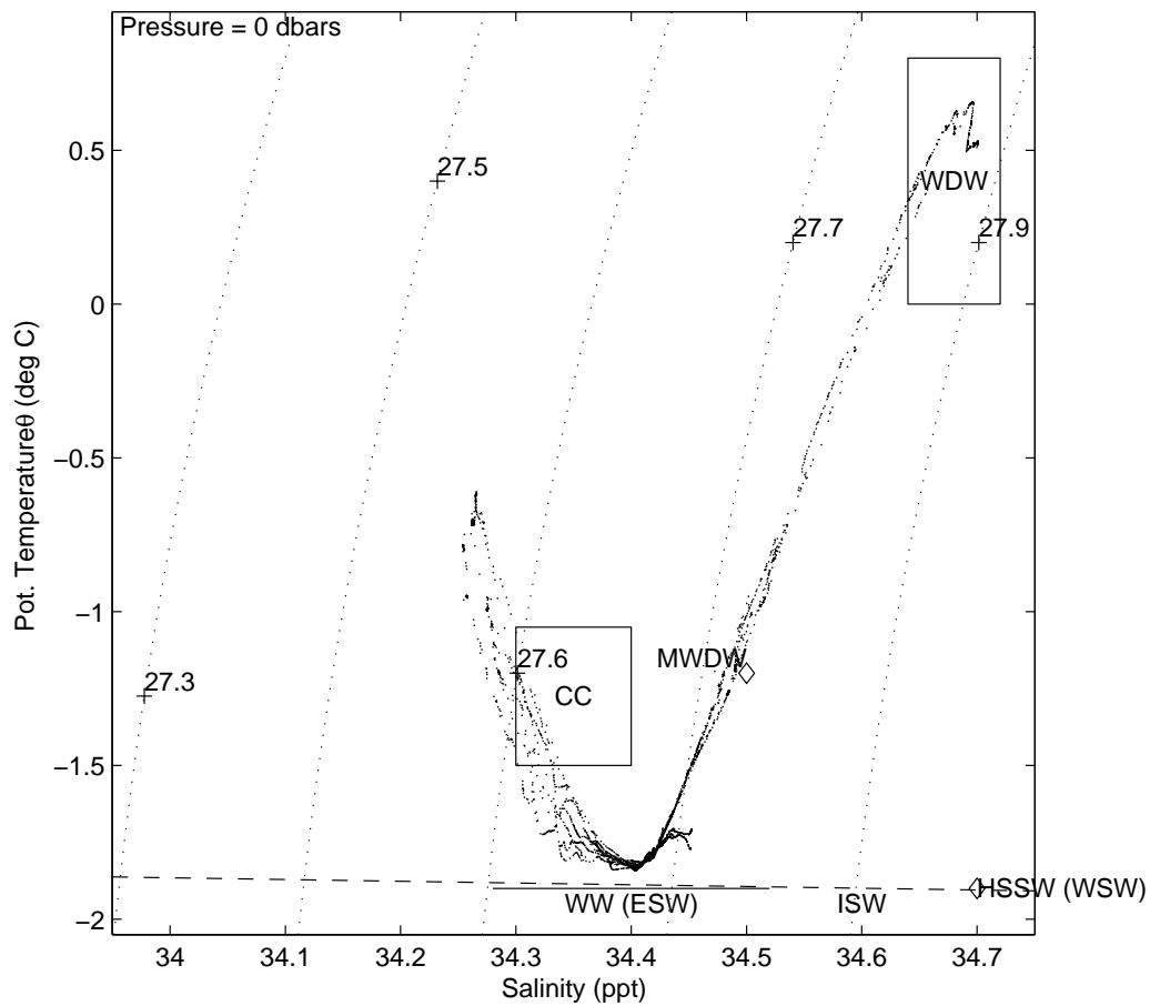
Fig. 24. \theta - S diagram from section 8.
