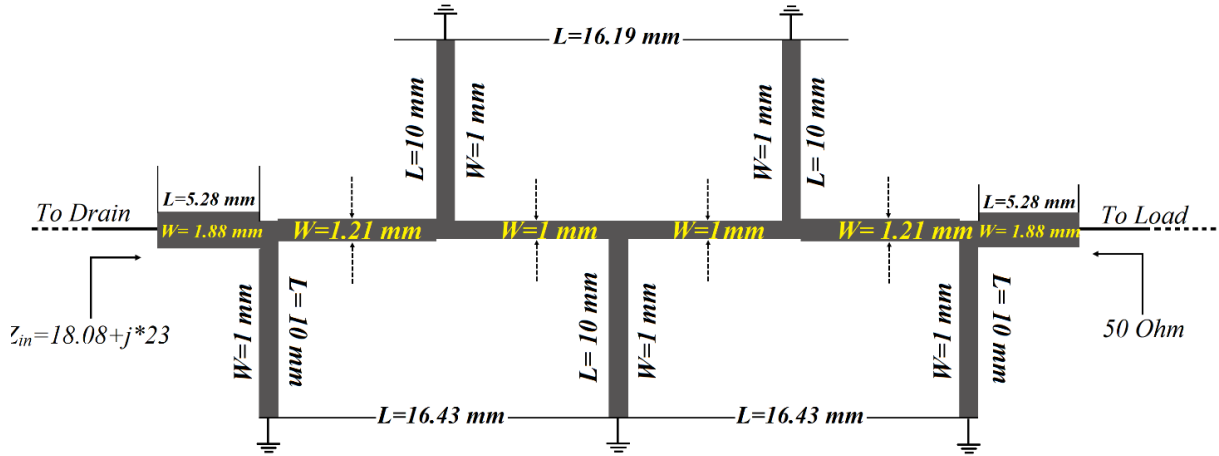
Fig. 4. The proposed broadband BPF uses a microstrip line
