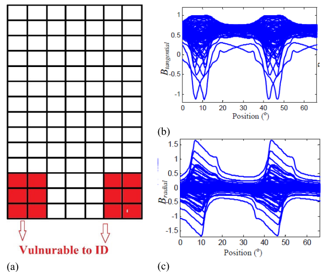
FIGURE 10. Flux density change waveform of each element at one PM versus rotor position (@16 C) (a) PM region drawing (b) tangential component (c) radial component [19].
