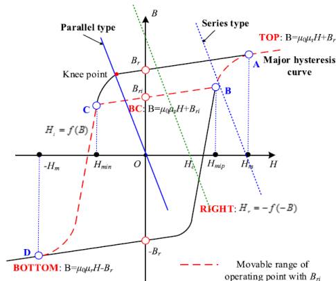
FIGURE 7. Numerical illustration of Fourier series-based hysteresis model [50].
