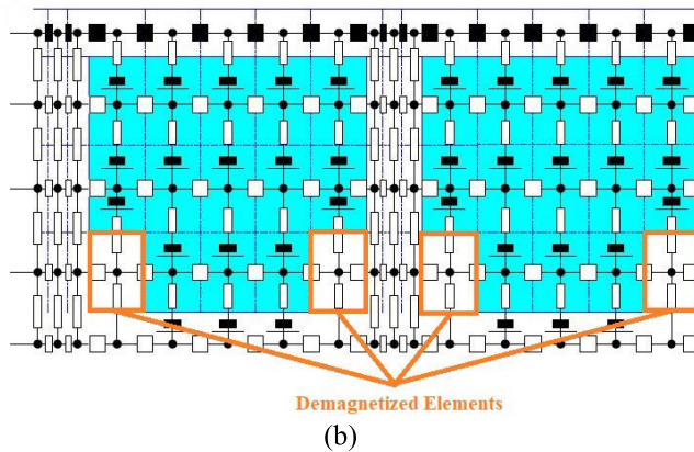
FIGURE 15. (a) The FEM model of the outer rotor SPM motor with symmetric demagnetized area and (b) The MEC model of the SPM motor with 4 demagnetized PM elements [69].
