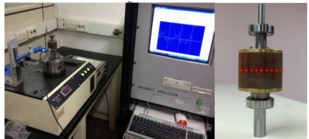
FIGURE 33. Experimental setup for ID analysis [53].
