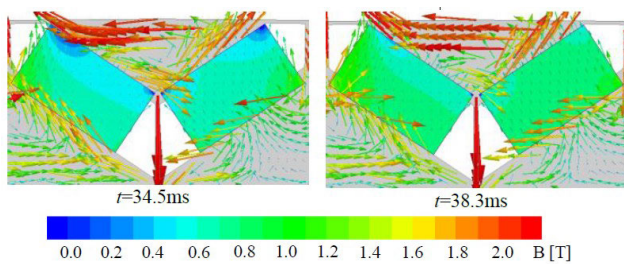
FIGURE 9. Flux density and vector distributions in different time instants [54].
