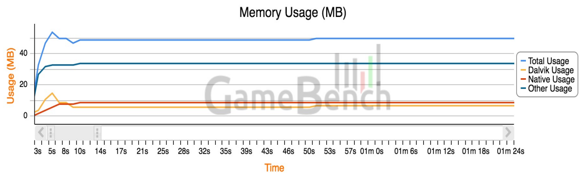
Figure 5.19: Stand Alone Version Performance - RAM
