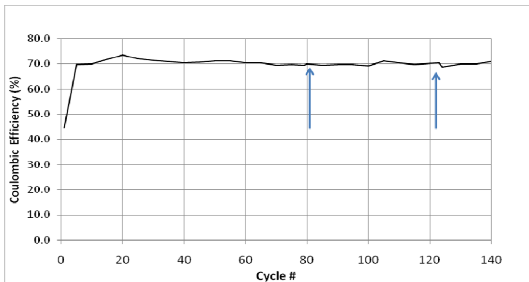
Figure 4-1-11: Coulombic efficiency for the main discharge plateau in a bare GF Al anode with oxide removed GF5 subjected to 140 cycles at a current density of 0.5 mA/cm 2 without an initial CV. Plateau jump events are indicated with arrows.
