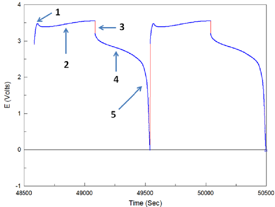
Figure 4-7-2: Characteristic features of galvanic cycles for lithiation-delithiation in a battery prototype setup with a solid polymer electrolyte, \text{LiFePO}_4 cathode and a GF Al anode at a current density of 0.065 \text{ mA/cm}^2 . Numbers indicate the features of interest: (1) potential overshoot (2) anode lithiation and cathode delithiation plateau (3) IR drop (4) anode delithiation and cathode lithiation plateau (5) discharge tail.
