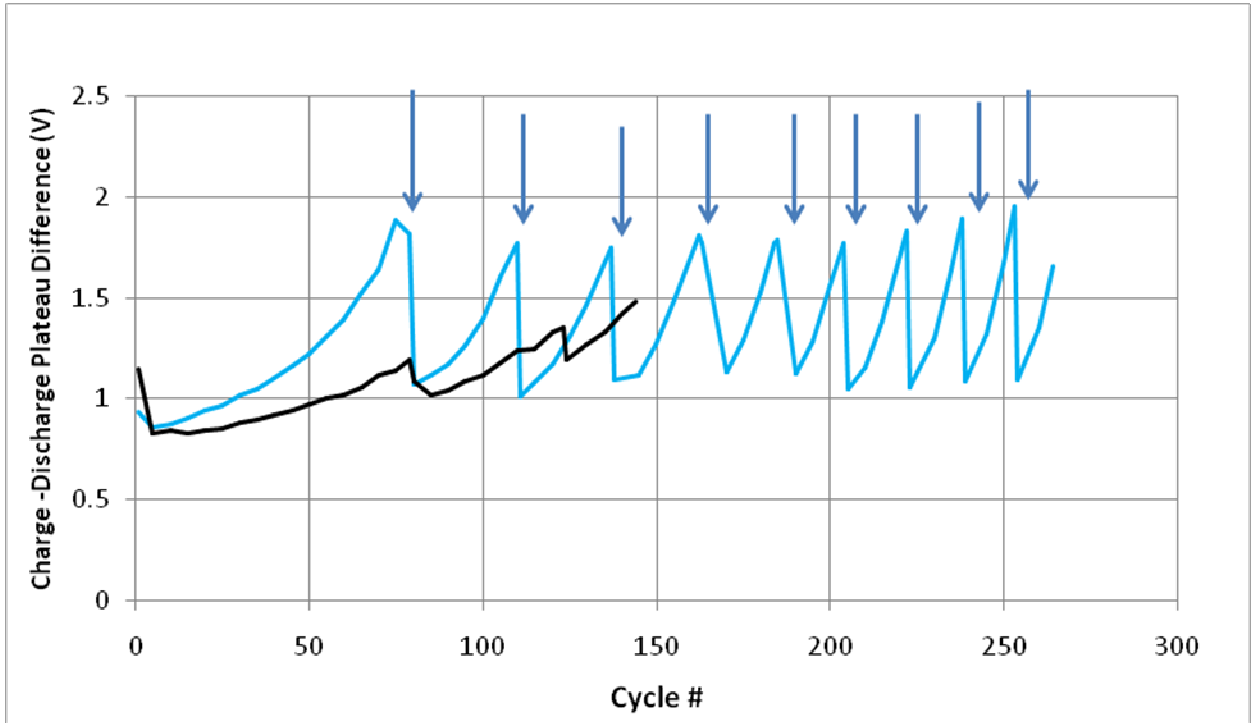
Figure 4-2-9: Charge-Discharge plateau separation (blue curve) for the main discharge plateau for MC3 soft MC Al anode with native oxide subjected to 264 cycles at a current density of 0.5 mA/cm 2 without an initial CV. For comparison, data for half-hard GF5 GF Al anode (oxide removed) from Ch. 4.1 are included in black. Plateau jump events in MC3 are indicated with arrows.
