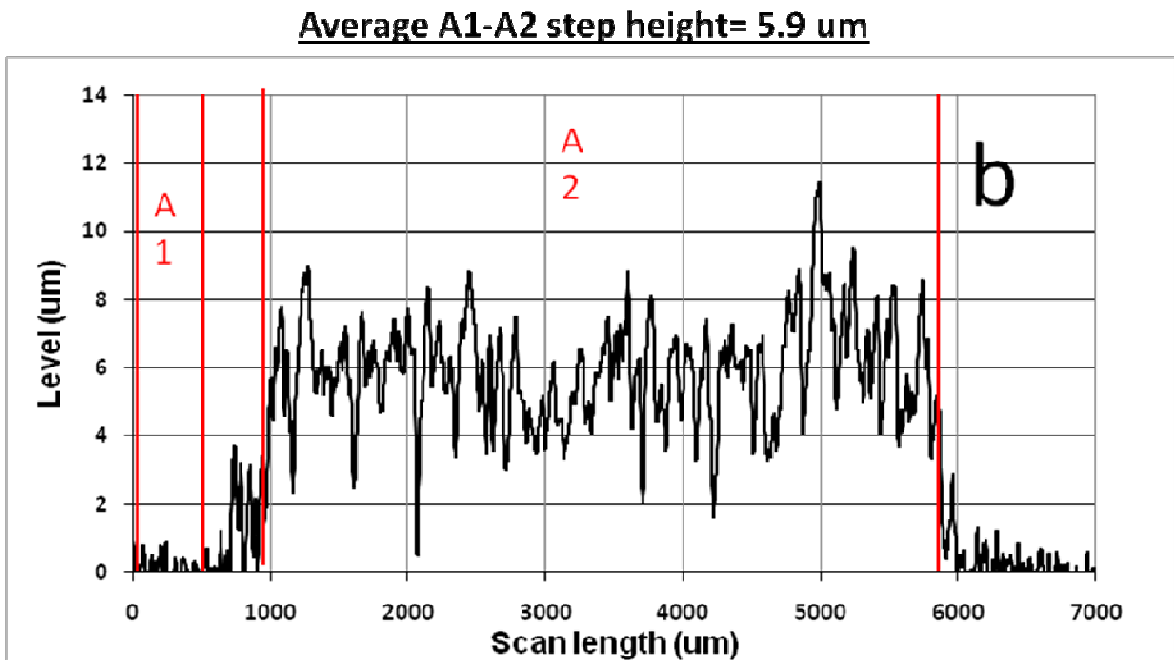
Fig. 4-6-11: Surface Profiles for (a) non-annealed AC1 and (b) annealed AC2 75% \text{N}_2 Al-CN x anodes after being subjected to 4x8 experiments in Ch. 4.4. Line scan is from gasket area to cycled area to gasket area. Step height is average difference of A1 and A2 areas.
