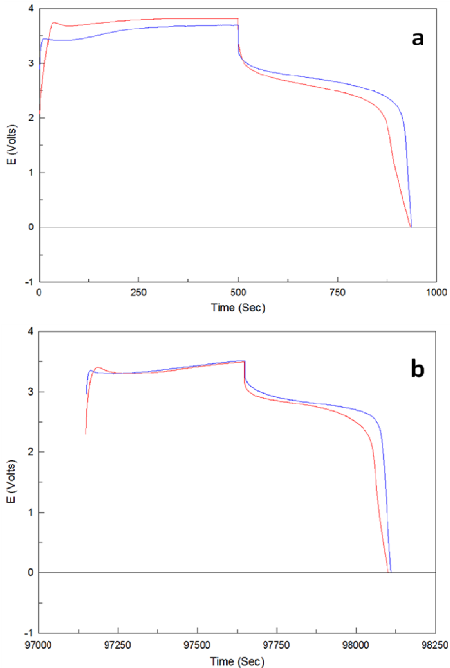
Figure 4-7-18: (a) Initial and (b) middle battery galvanic cycles of sample BAT4 with a solid polymer electrolyte, LiFePO 4 cathode and a non-annealed 25% N 2 75 nm Al-CN x anode at current densities of 0.065 (red) and 0.13 (blue) mA/cm 2 . For both current densities cycling was performed for 200 cycles each with charge/discharge times of 500 seconds. Cycles have been offset in figure b to overlap the curves on the same time scale.
