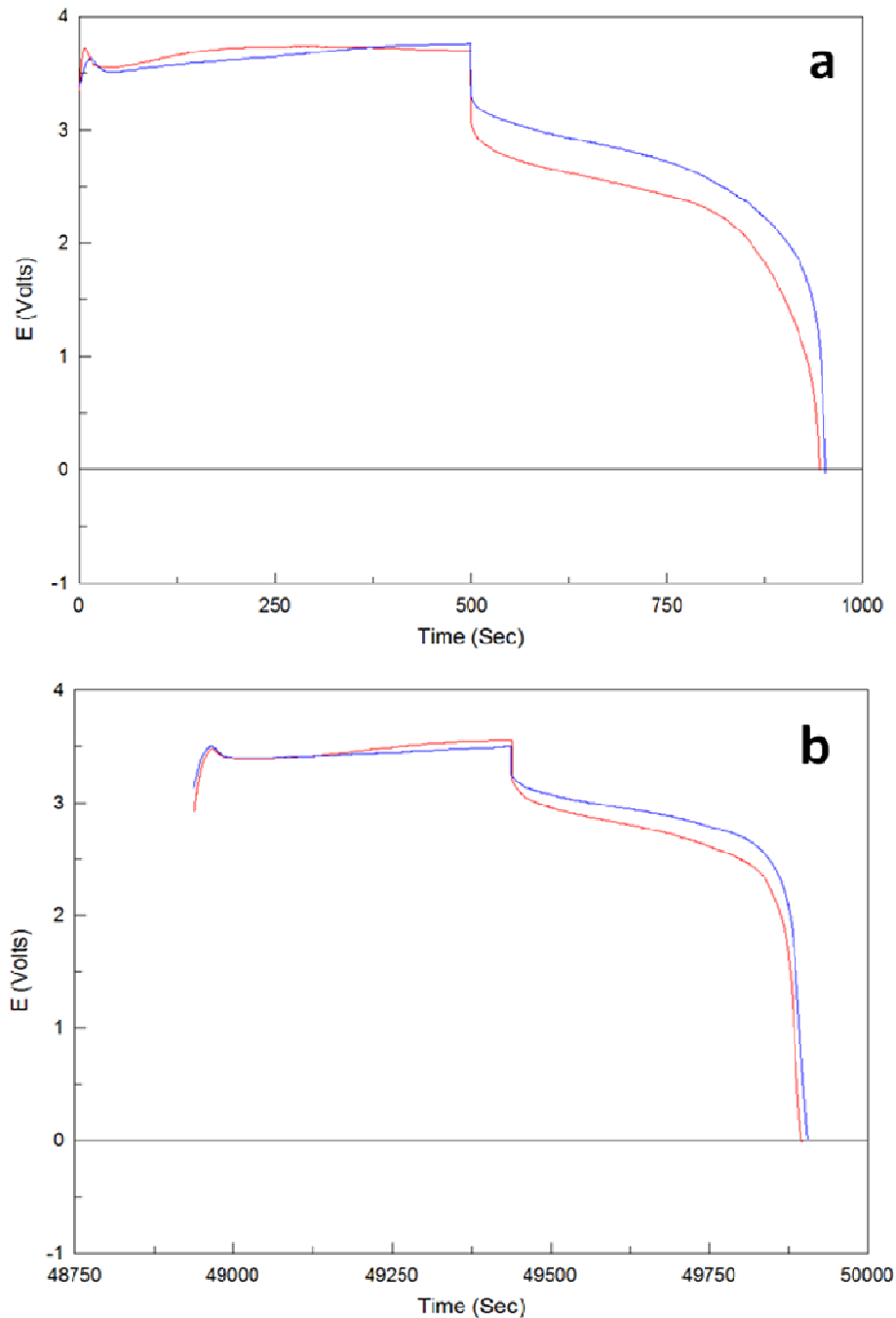
Figure 4-7-6: (a) Initial and (b) middle battery galvanic cycles of sample BAT1 with a solid polymer electrolyte, LiFePO 4 cathode and a bare polish + etch GF Al anode at current densities of 0.065 (red) and 0.13 (blue) mA/cm 2 . For both current densities cycling was performed for 100 cycles each with charge/discharge times of 500 seconds. Cycles have been offset in figure b to overlap the curves on the same time scale.
