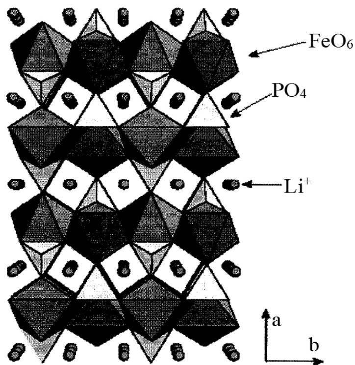
Figure 2-4-2: The crystal structure of olivine LiFePO 4 , from ref. 41.
