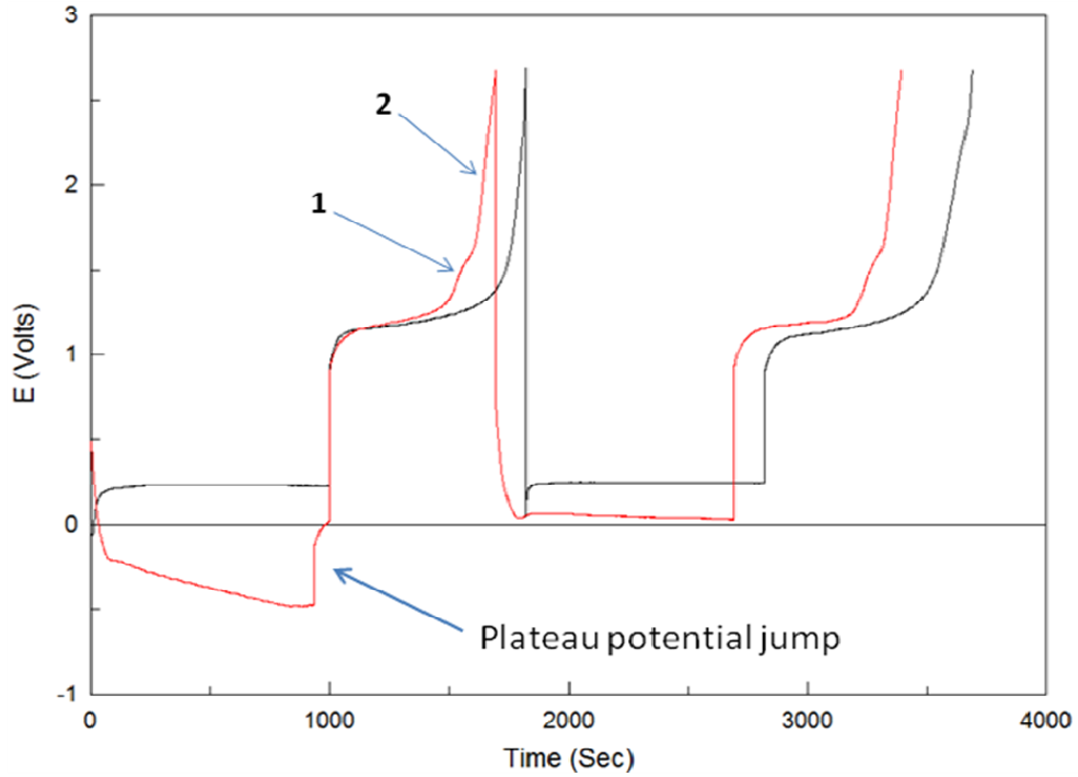
Figure 4-2-8: First two (black) and last two (red) galvanic cycles for the MC3 soft MC Al anode with native oxide subjected to 264 cycles at a current density of 0.5 \text{ mA/cm}^2 without an initial CV. Numbers in the red curve denote the secondary and tertiary diffusion-limited plateaus. The red curve has been offset to overlap with the time scale of the black curve.
