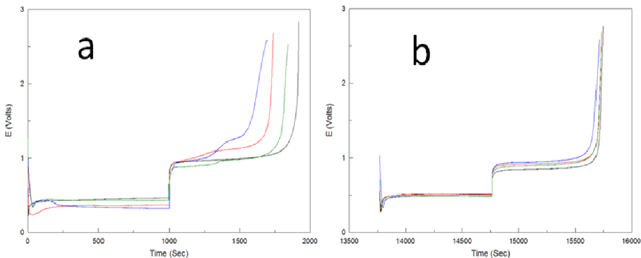
Figure 4-5-5: (a) First and (b) last galvanic cycles of Al-Al and non-annealed and annealed Al-Al-CN x anodes ACM1 (red), ACM2 (blue) and ACM3 (green) at a current density of 0.13 mA/cm 2 . Comparative bare half-hard GF Al anode GF1 (oxide removed) from Ch. 4.1 is also included (black). Cycles in the right figure have been offset to overlap the curves on the same time scale.
