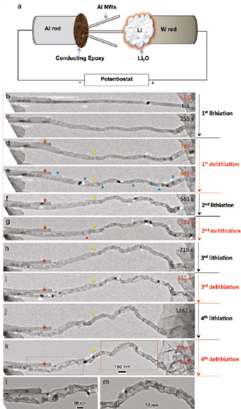
Figure 2-3-7: Pulverization of a single aluminum NW upon electrochemical cycling, from ref. 19.
