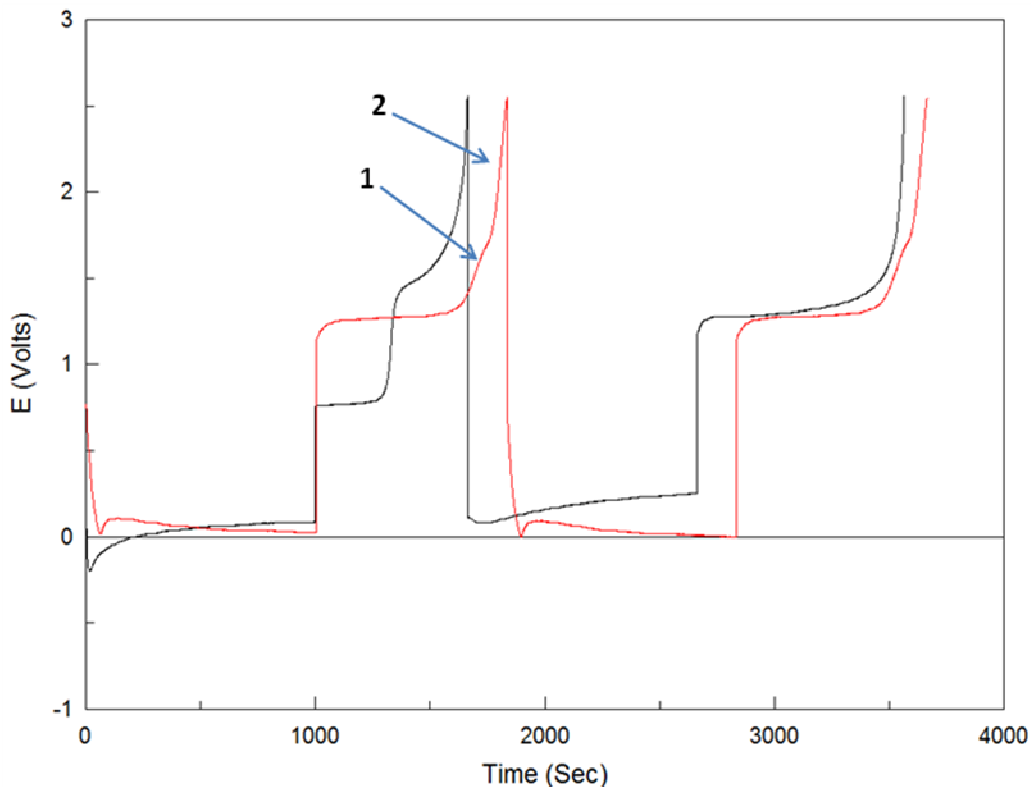
Figure 4-4-8: First two (black) and last two (red) galvanic cycles for the AC3 non-annealed 75% N 2 Al-CN x anode subjected to 180 cycles at a current density of 0.5 mA/cm 2 without an initial CV. Numbers in the red curve denote the secondary and tertiary diffusion-limited plateaus. The red curve has been offset to overlap with the time scale of the black curve.
