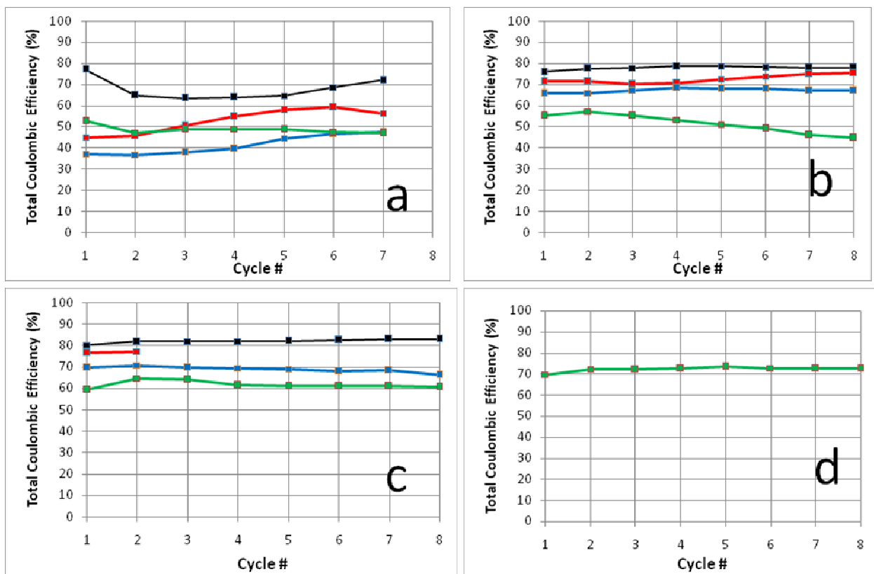
Figure 4-5-8: Coulombic efficiencies of non-annealed and annealed 25+75 nm Cu-Al-CN x anodes CM1 (black) and CM2 (red), non-annealed 75+25+75 nm and 25+75+50 nm Cu-CN x -Al-CN x anodes CM3 (blue) and CM4 (green) at current densities of (a) 0.13 (b) 0.25 (c) 0.5 and (d) 1 mA/cm 2 . All lithiation/delithiation processes have been summed together for calculation of the coulombic efficiency.
