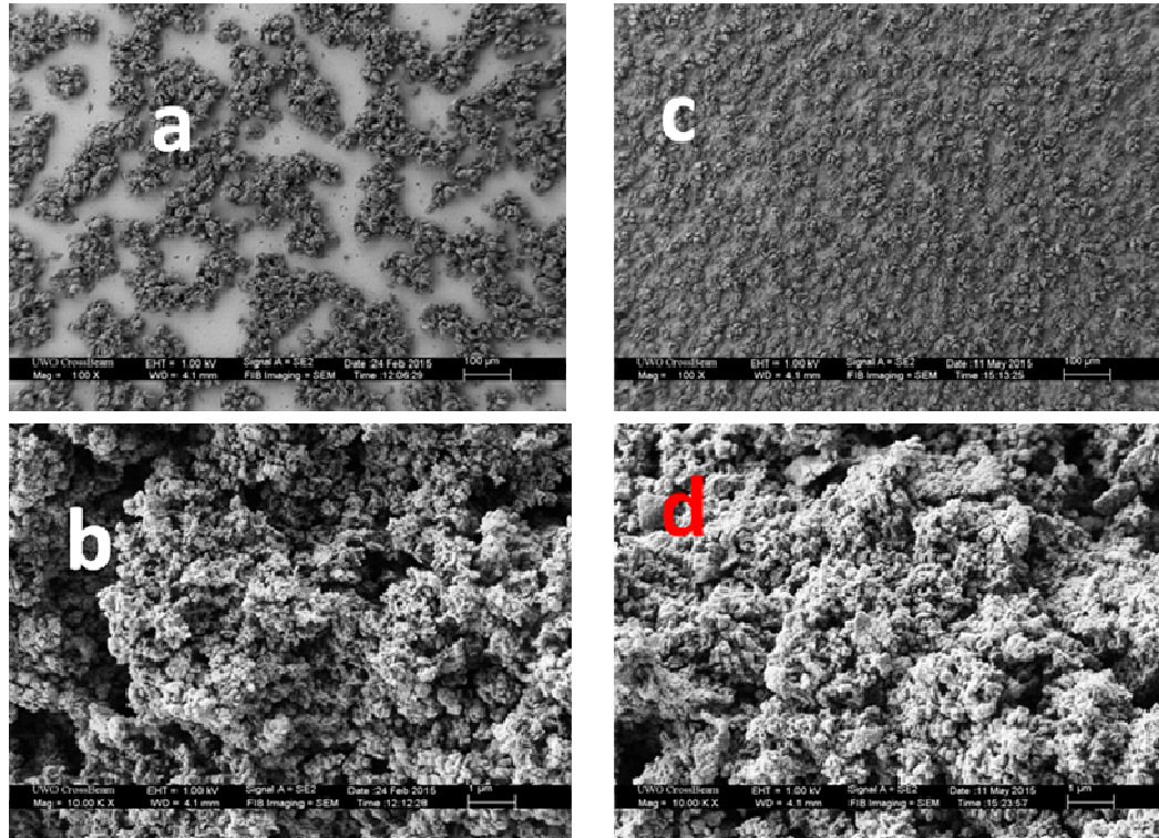
Figure 4-4-27: SEM images of cycled areas for (a-b) non-annealed 75% N 2 (DC1) Dural-CNx, (c-d) non-annealed 25% N 2 (DC2) Dural-CNx anodes. Magnifications of (a,c) 100x, (b,d) 10000x.
