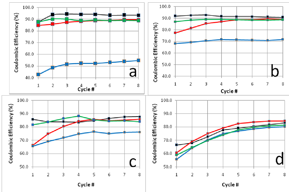
Figure 4-2-6: Coulombic efficiencies of two soft MC Al anodes MC1 and MC2 prepared with varying degrees of surface oxide remaining at current densities of (a) 0.13 (b) 0.25 (c) 0.5 and (d) 1 mA/cm 2 . Comparative half-hard GF Al anodes GF1 and GF4 from Ch. 4.1 are included. Samples GF1 (hard, oxide removed), MC1 (soft, oxide removed), MC2 (soft, native oxide) and GF4 (hard, native oxide) are in black, red, blue and green colors, respectively.
