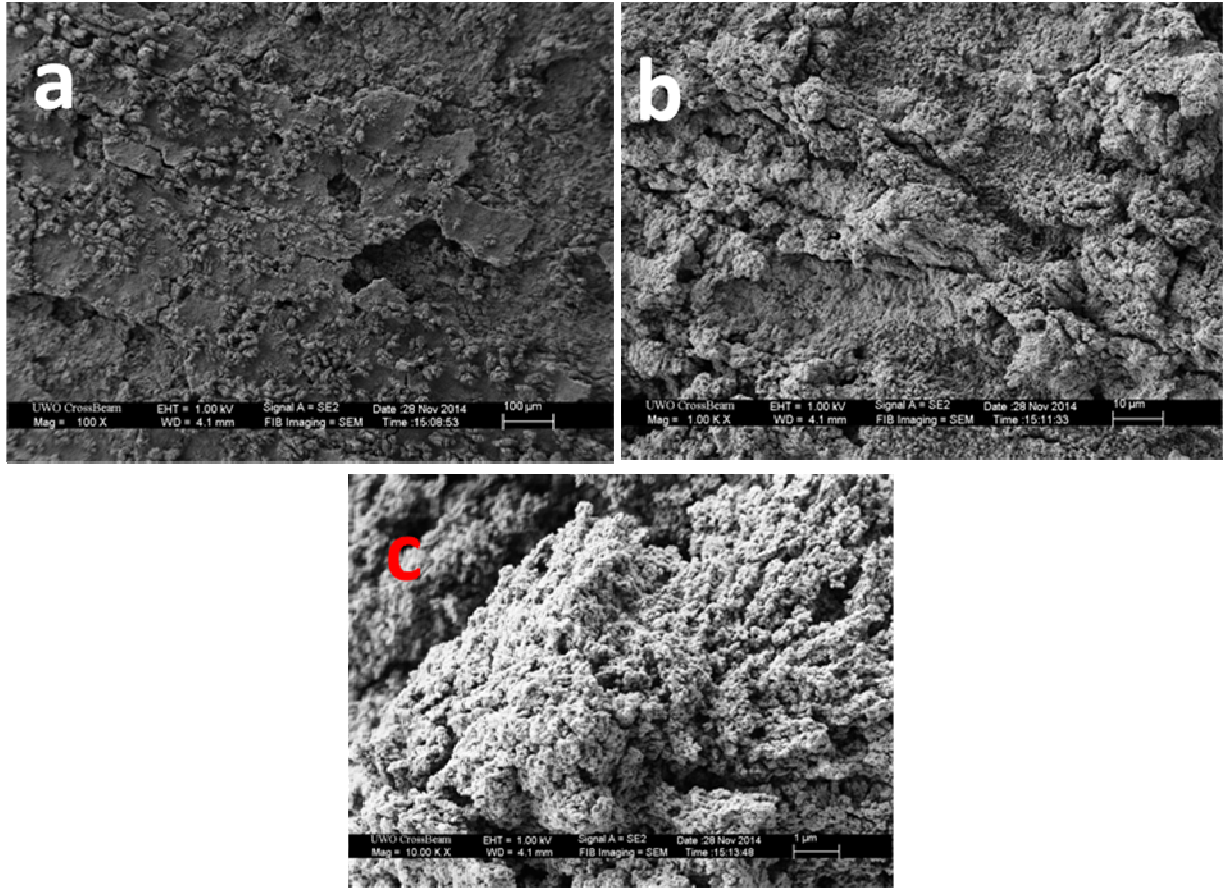
Figure 4-2-13: SEM images of cycled area for soft MC Al anode with native oxide MC3 after being subjected to 264 cycles at a current density of 0.5 \text{ mA/cm}^2 without an initial CV. Magnifications of (a) 100x (b) 1000x (c) 10000x.
