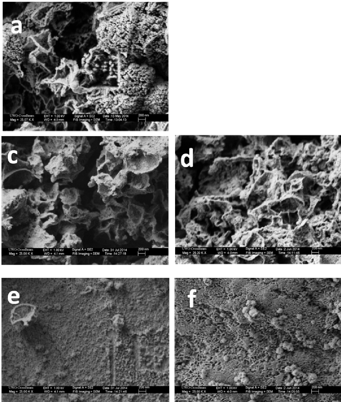
Figure 4-5-15: SEM images of cycled areas from 4x8 experiments for (a) non-annealed 75% N 2 25+75 nm Cu-Al-CNx (CM1), (c,e) non-annealed 75% N 2 25+75+50 nm Cu-CNx-Al-CNx (CM4) two areas, (d,f) non-annealed 75% N 2 75+25+75 nm Cu-CNx-Al-CNx (CM3) two areas. Magnifications of 25000x.
