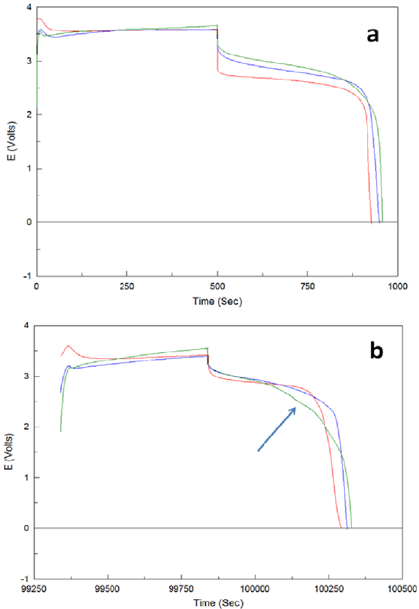
Figure 4-7-10: (a) Initial and (b) middle battery galvanic cycles of sample BAT2 with a solid polymer electrolyte, LiFePO 4 cathode and a non-annealed 75% N 2 75 nm Al-CN x anode at current densities of 0.065 (red), 0.13 (blue) and 0.32 (green) mA/cm 2 . For all current densities cycling was performed for 200 cycles each with charge/discharge times of 500 seconds. Cycles have been offset in figure b to overlap the curves on the same time scale. Arrow in green curve of figure b indicates appearance of secondary diffusion-limited discharge plateau.
