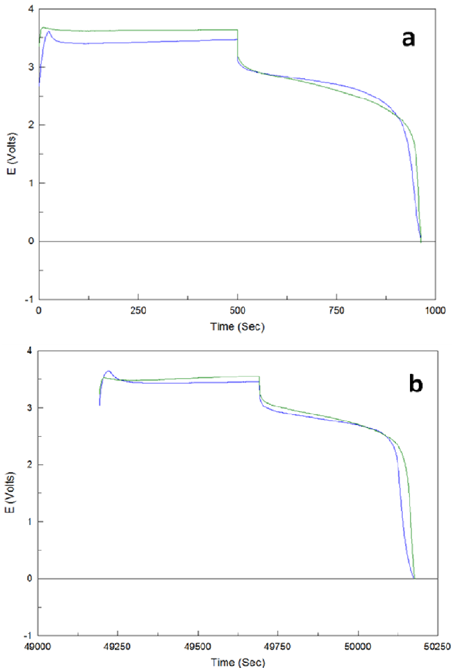
Fig. 4-7-22: (a) Initial and (b) middle battery galvanic cycles of sample BAT5 with a solid polymer electrolyte, LiFePO 4 cathode and a non-annealed 75% N 2 75 nm Al-CN x anode at current densities of 0.065 (blue) and 0.13 (green) mA/cm 2 . For both current densities cycling was performed for 100 cycles each with charge/discharge times of 500 seconds. Cycles have been offset in figure b to overlap the curves on the same time scale.
