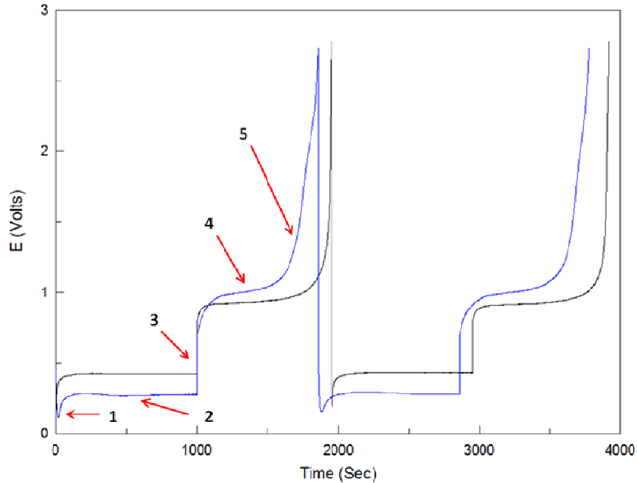
Figure 4-3-3: Typical galvanic cycles for lithiation/delithiation of a Dural anode (blue curve). This is sample DU1 which was subjected to polishing and etching in acidic conditions prior to electrochemical scans. Comparative data for half-hard GF Al anode GF1 from Ch. 4.1 are also included (black curve). Numbers indicate the features of interest: (1) potential overshoot (2) charge plateau (3) IR drop (4) discharge plateau (5) discharge tail. Galvanic cycles are shown at a current density of 0.25 \text{ mA/cm}^2 .
