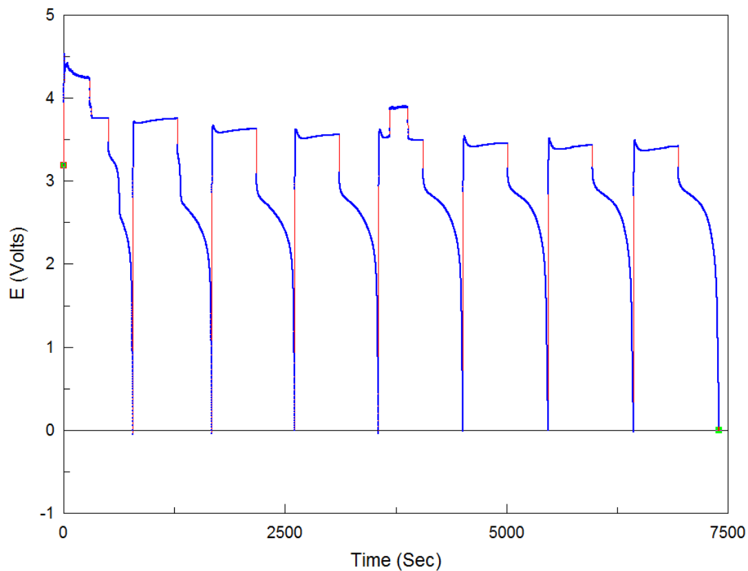
Figure 4-7-11: Full set of battery galvanic cycles of sample BAT3 with a solid polymer electrolyte, \text{LiFePO}_4 cathode and an annealed 75% \text{N}_2 75 nm Al-CN x anode at a current density of 0.033 \text{ mA/cm}^2 for 8 cycles with charge/discharge times of 500 seconds each.
