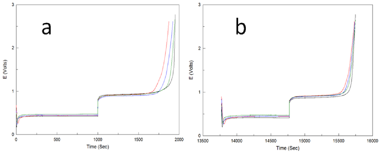
Figure 4-1-6: (a) First and (b) last galvanic cycles of four GF Al anodes prepared with varying degrees of surface oxide remaining at a current density of 0.25 \text{ mA/cm}^2 . Samples GF1 (oxide removed), GF2 (polished only), GF3 (additional oxide) and GF4 (native oxide) in black, red, blue and green respectively. Cycles in the right figure have been offset to overlap the curves on the same time scale.
