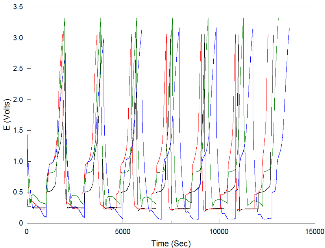
Figure 4-5-7: Galvanic cycles for non-annealed and annealed 75% N 2 25+75 nm Cu-Al-CN x anodes CM1 (black) and CM2 (red), non-annealed 75% N 2 75+25+75 nm and 25+75+50 nm Cu-CN x -Al-CN x anodes CM3 (blue) and CM4 (green), at a current density of 0.13 mA/cm 2 .
