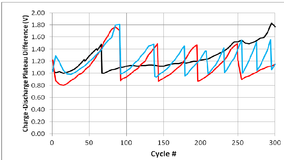
Figure 4-4-20: Charge-Discharge plateau separation for the main discharge plateau for non-annealed DC3 75% N 2 (red curve) and DC4 25% N 2 (blue curve) Dural-CN x anodes subjected to 300 cycles each at a current density of 0.5 mA/cm 2 without an initial CV. For comparison, data for bare DU2 Dural anode (oxide removed) from Ch. 4.3 is included in black.
