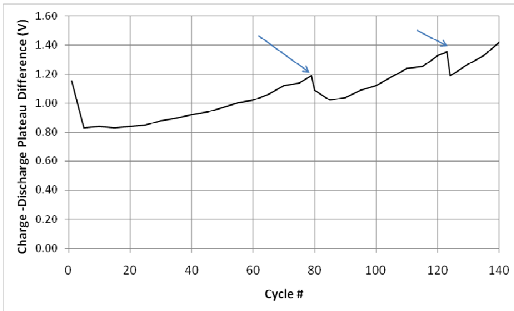
Figure 4-1-10: Charge-Discharge plateau separation for the main discharge plateau in a bare GF Al anode with oxide removed GF5 subjected to 140 cycles at a current density of 0.5 mA/cm 2 without an initial CV. Plateau jump events are indicated with arrows.
