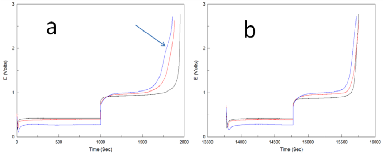
Figure 4-3-5: (a) First and (b) last galvanic cycles of Dural anode DU1 (blue) prepared with oxide removed at a current density of 0.25 \text{ mA/cm}^2 . Comparative data for half-hard GF Al (black) and soft MC Al (red) anodes GF1 and MC1 from Ch. 4.1 and 4.2 are also included. Cycles in the right figure have been offset to overlap the curves on the same time scale. Arrow indicates appearance of diffusion-limited discharge plateau in DU1.
