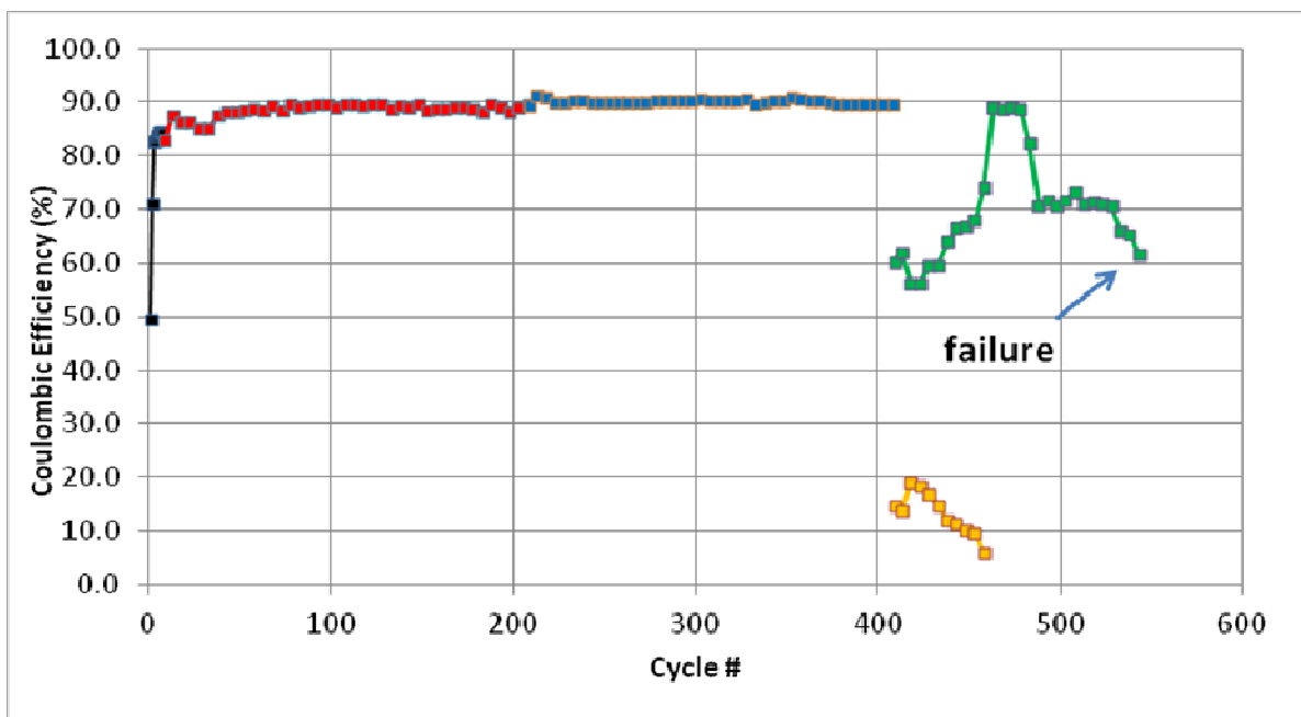
Figure 4-7-12: Coulombic efficiency for the main discharge plateau in battery galvanic cycles of sample BAT3 with a solid polymer electrolyte, \text{LiFePO}_4 cathode and an annealed 75% \text{N}_2 75 nm Al-CN x anode at current densities of 0.033 (black), 0.065 (red), 0.13 (blue) and 0.32 (green) \text{mA}/\text{cm}^2 . Yellow curve shows coulombic efficiency of secondary diffusion-limited discharge plateau at 0.32 \text{mA}/\text{cm}^2 . Horizontal axis shows the cumulative number of cycles of all sets together. The arrow in the green curve indicates the onset of battery failure.
