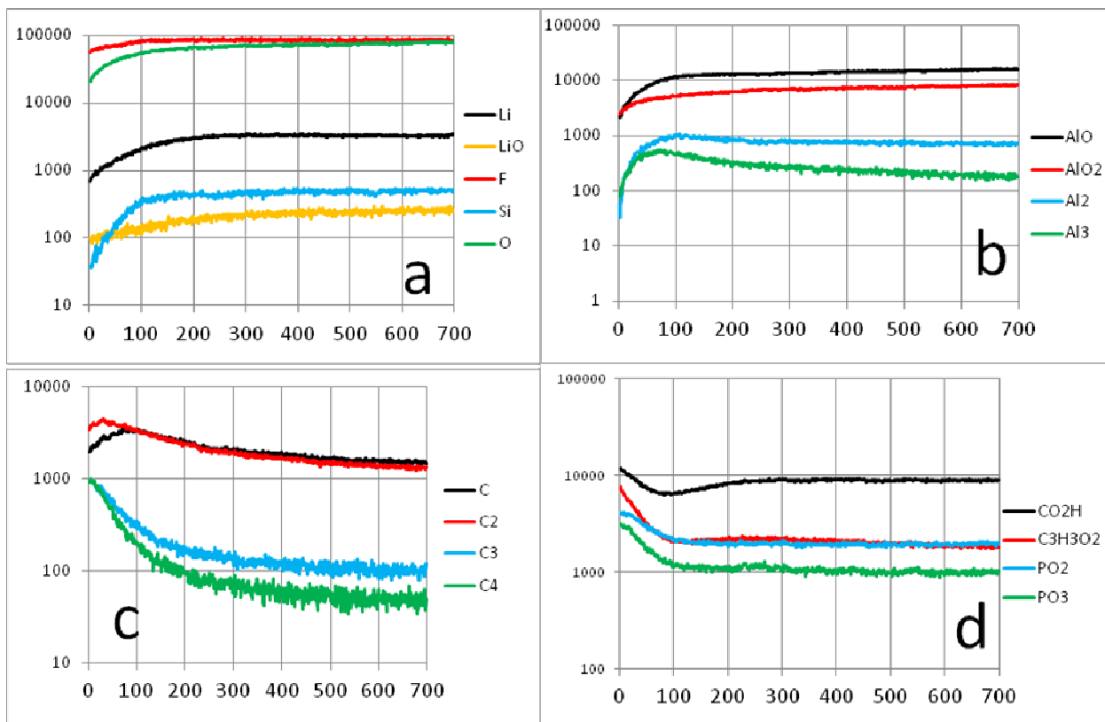
Figure 4-6-2: TOF-SIMS negative secondary ion depth profiles of cycled area for bare half-hard Goodfellow Al anode GF1 (oxide removed) subjected to 4x8 experiment from Ch. 4.1. Vertical axis is raw ion intensity counts. Horizontal axis is total active time in seconds for Cs + sputter beam.
