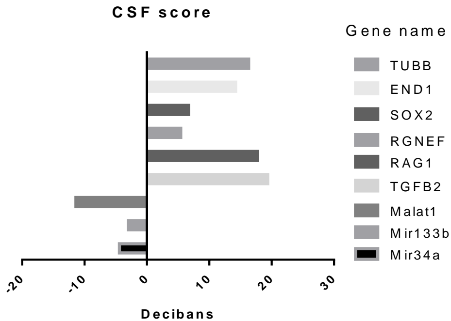
Figure 3.3: CSF scores
